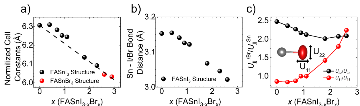
Figure 5: a) The normalized unit cell constants, based on single crystal X-ray diffraction data, for each compound synthesized in the \text{FASnI}_{3-x}\text{Br}_x ( x = 0 - 3 ) system. Compounds are labeled by their structure type in black and red for the \text{FASnI}_3 ( Pm\bar{3}m ) and \text{FASnBr}_3 ( Pa\bar{3} ) structure type, respectively. The dashed line displays the ideal behavior based on Vegard's Law analysis. b) The bond distances for each compound with the \text{FASnI}_3 structure plotted against composition. c) A plot of the U_{11} (red) and U_{22} (black) anisotropic displacement parameters as a function of composition normalized to the displacement parameters of the central Sn considering the same direction for all \text{FASnI}_{3-x}\text{Br}_x compounds that retain the \text{FASnI}_3 cubic structure. Note that the U_{22} and the U_{33} parameters are equivalent for both the halide and metal atoms.
