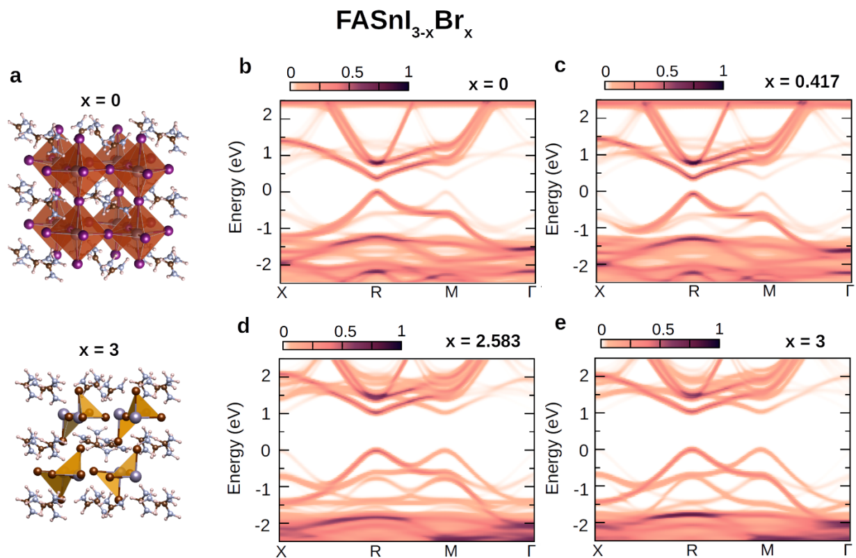
Figure S13: Electron spectral functions of FASnI 3-x Br x . (a) DFT optimized structures of cubic FASnI 3 ( x = 0 ) and FASnBr 3 ( x = 3 ) accounting for local disorder (polymorphism). 3,4 (b-e) DFT electron spectral functions (color map) of FASnI 3-x Br x for x = 0 (b), x = 0.417 (c), x = 2.583 (d), and x = 3 (e) calculated using band structure unfolding 5,6 and the PBEsol approximation.
