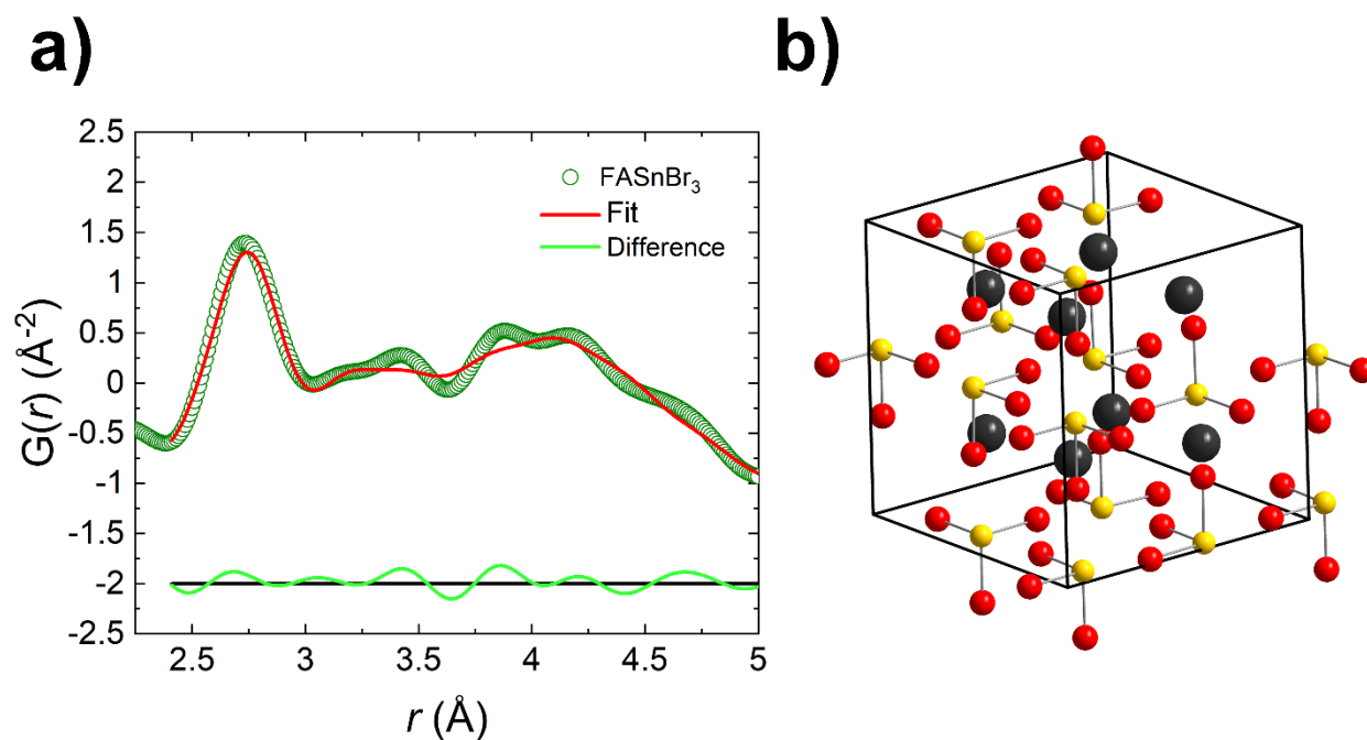
Figure S7: a) Experimental and theoretical G(r) curves as well as the difference curve within the range of 2.5-5 Å. b) the refined local structure model of \text{FASnBr}_3 . The space group symmetry was relaxed to P1 for the model.
