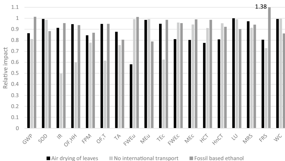
Fig. 5 Relative impact change of altering parameters within the life cycle inventory; air drying of leaves (black), no international transport (light grey) and ethanol derived from fossil sources instead of fermentation (dark grey) are shown. FRS for fossil-based ethanol is greater than 1.1, at a value of 1.38 (marked on graph)
