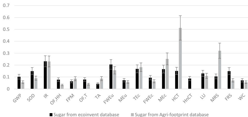
Fig. 6 Relative impact of 1 kg SE RA60 to a global mix of sugar (impact = 1 for each impact category), for sugar within the ecoinvent 3.8 database (black) and the Agri-footprint 6.1 database (grey). Effect of sweetness equivalence variation between 200 and 300 shown as error bars on RA60 data
