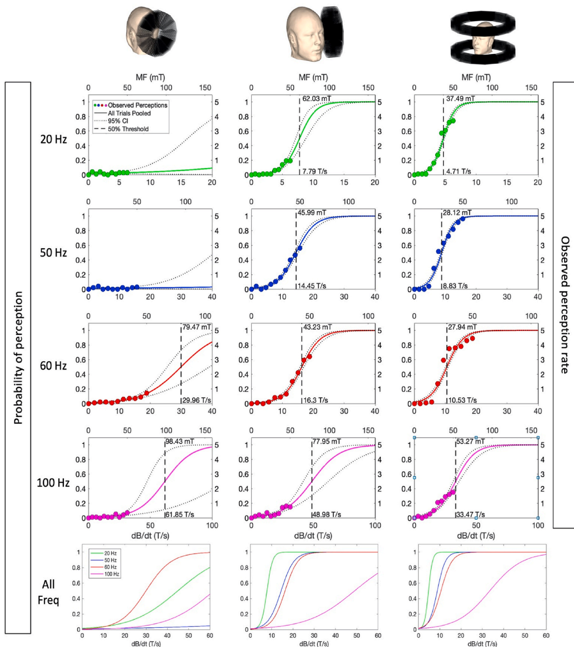
Fig. 1. Top 4 Rows: For each frequency-exposure modality combination, the colored dots represent the mean observed magnetophosphene perception rates vs dB/dt (bottom x -axes) and B (top x -axes) pooled across Trials . These data points are shown with the logistic regression curves broken out by Trial with their collective 95 % CI . Bottom Row: The mean magnetophosphene perception curves pooled across Trials for each frequency. Vertical axis: probability (or rate) of perception; bottom x -axis: dB/dt in Tesla per second (T/s); top x -axis: B in Tesla (T). The field values shown along the bottom (top) x -axes indicate dB/dt ( B ) corresponding to a 50 % response rate.
