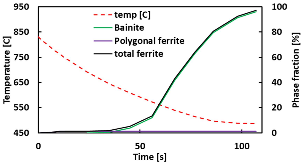
Figure 8. In-situ temperature paths and estimated bainite fraction during cooling.
