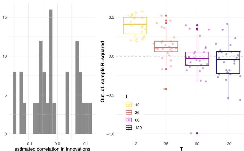
Fig. 8. VIX prediction. In the left panel, we show the distribution of estimated correlations between innovations of the VIX and innovations for all other predictors. In the right panel, we plot the out-of-sample R^2 stemming from PRs in which the VIX is the dependent variable. All other predictors are used, one at a time, except the svar. Before averaging, we remove all outliers in predictions, i.e. those values that lie outside the [0\%, +500\%] interval. Each point corresponds to one predictor and one calendar decade (over which the R^2 is computed).
