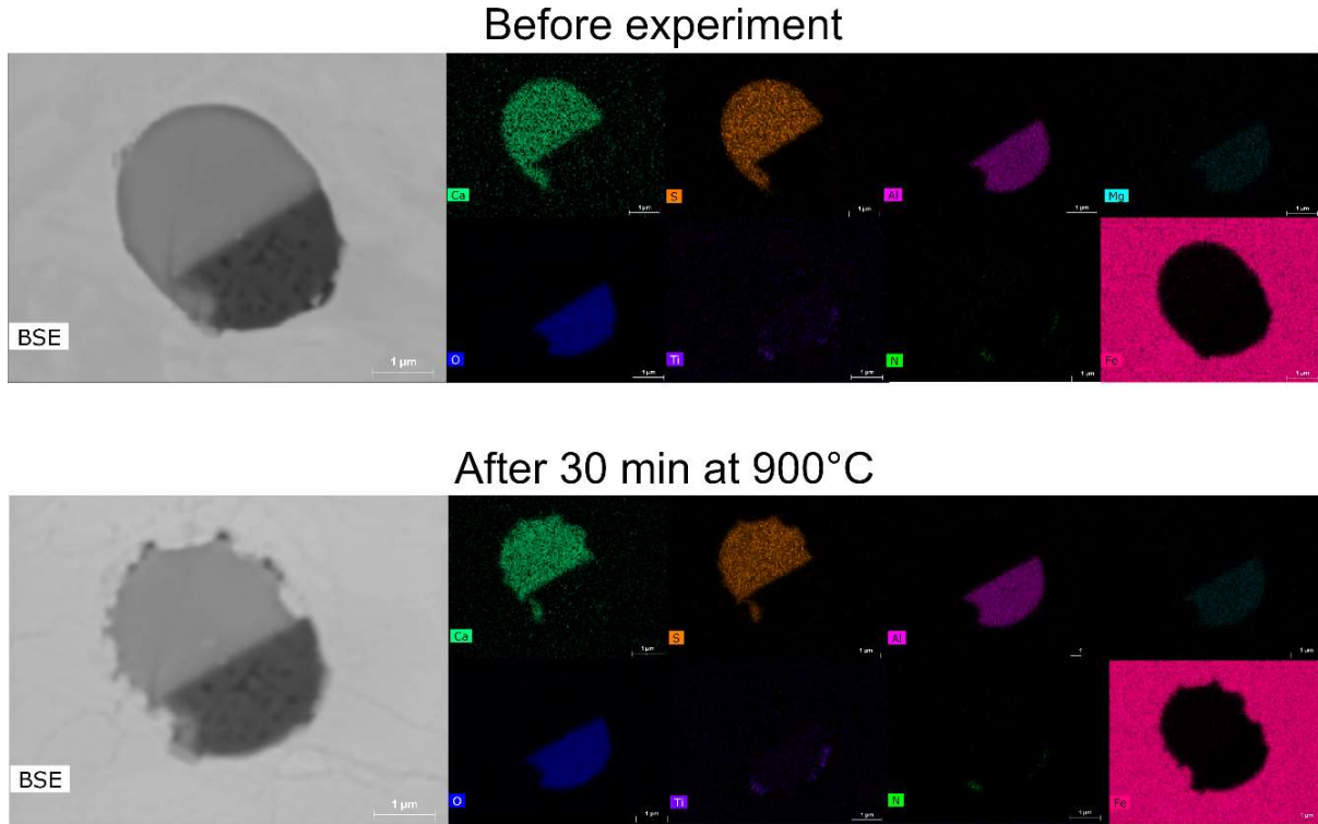
Figure 4. Spinel–CaS type NMI before and after experiment, BSE images and elemental maps.
