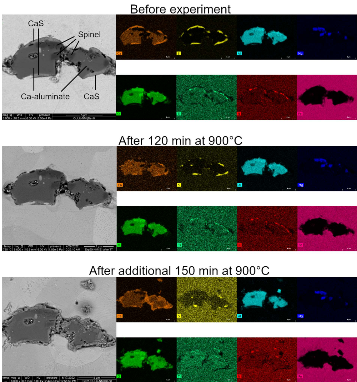
Figure 1. Complex calcium aluminate NMI before and after experiment, BSE images and elemental maps.
