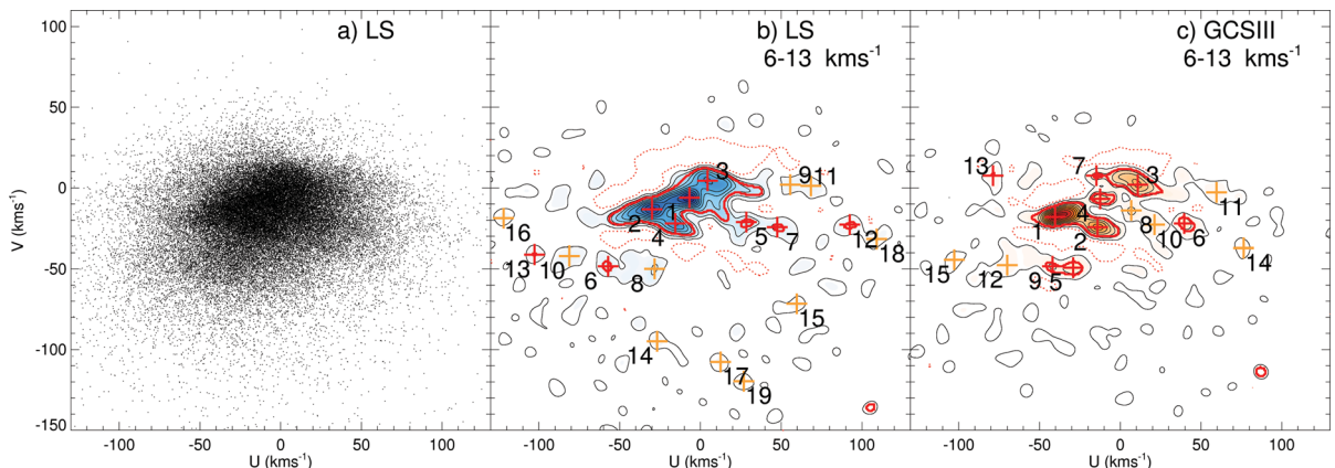
Figure 2. (a) Heliocentric velocities of the local sample (LS). (b) Velocity structures in the local sample (LS) obtained with the wavelet transform at scales of 6\text{--}13\text{ km s}^{-1} . The red solid (dotted) contour shows the 3\sigma confidence limit for positive wavelet coefficients or overdensities (negative coefficients or underdensities). Red (orange) crosses show the maxima of the detected peaks inside the 3\sigma ( 2\sigma ) confidence limit. (c) Same as (b), but for GCSIII sample.
