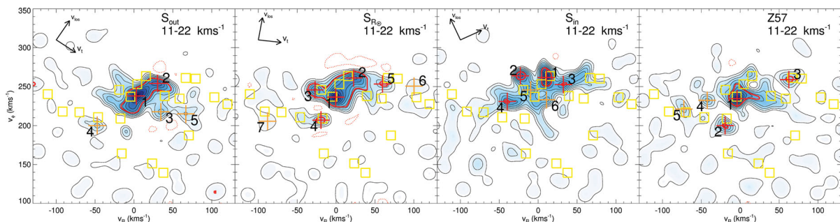
Figure 3. Velocity structures at scales of 11–22 km s ^{-1} in cylindrical velocities for the subsamples S_{\text{out}} (outside solar circle), S_{R_{\odot}} (solar circle), S_{\text{in}} (inside solar circle) and Z57 ( -700 \leq Z \leq -500 pc). Yellow squares show the positions of the local sample (LS) groups. Colour code is the same as in Fig. 2(b).
