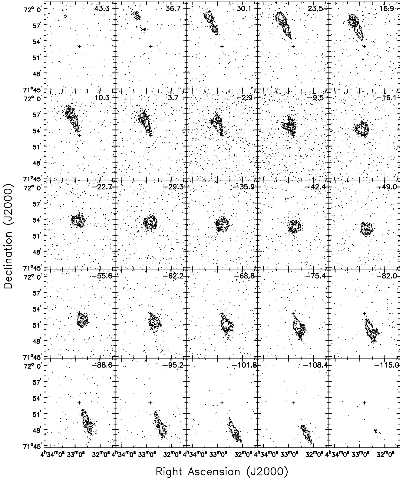
Figure 1. Observed channel maps of NGC 1560. The heliocentric radial velocity (in \text{km s}^{-1} ) is indicated at the top right-hand corner of each channel map. Contours are -2.5, 2.5 ( \sim 3\sigma ), 5, 10, 20 and 40 \text{ mJy beam}^{-1} . The cross shows the location of the galaxy centre. The synthesized beam is 8.1 \times 6.4 \text{ arcsec}^2 .
