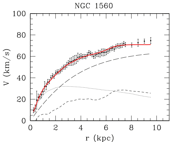
Figure 10. Rotation curve fit using the Burkert halo. Short-dashed, dotted, and long-dashed lines represent the Newtonian contributions of the gaseous disc, stellar disc and dark halo, respectively. The best-fitting model is shown as a solid red line.
