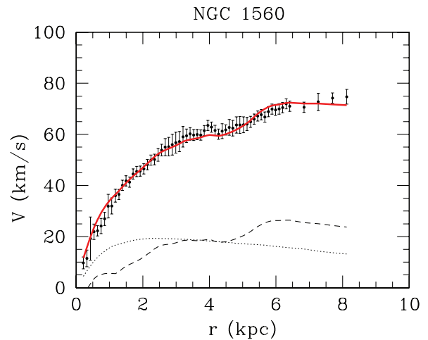
Figure 12. Rotation curve fit using MOND. The best-fitting distance is 2.94 Mpc. Lines and symbols are like those in Fig. 10.
