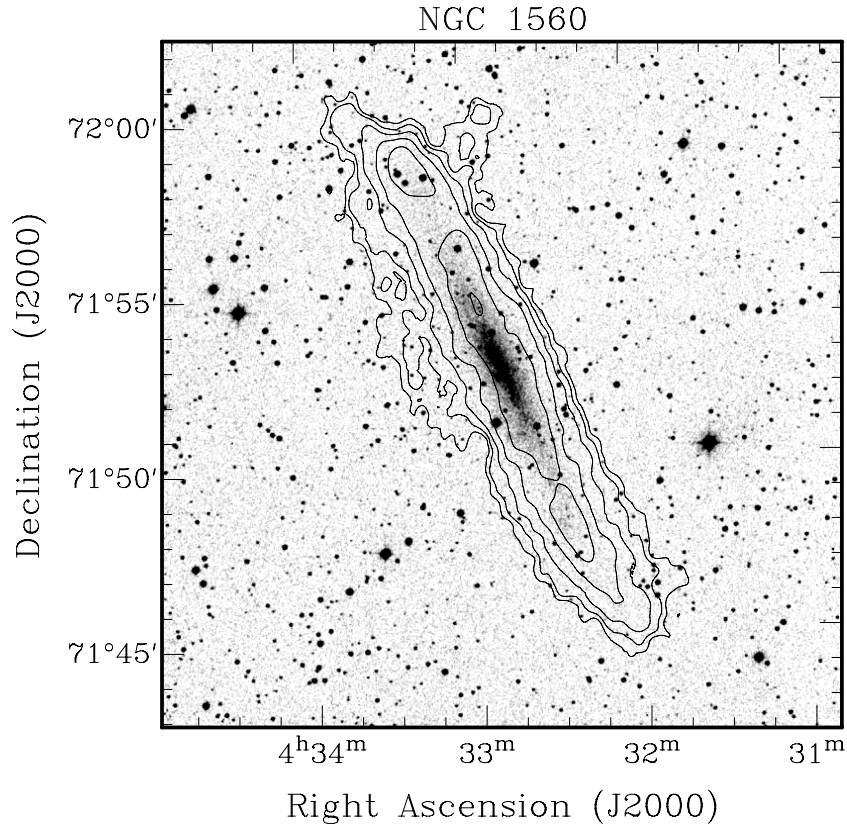
Figure 3. Total H I map based on the low-resolution data cube, overlaid with an optical (DSS) image. Contours are (1, 2, 4, 8, 16, 32, 64) \times 10^{20} atom \text{cm}^{-2} . The lowest contour represents the ‘pseudo- 3\sigma ’ level defined in the same way as Verheijen & Sancisi (2001). The synthesized beam is 25 \times 25 arcsec ^2 .
