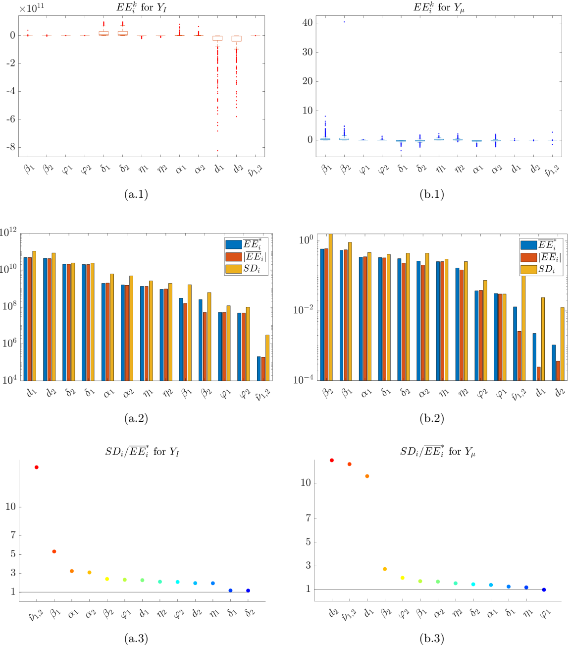
Figure S.5: Results of the Elementary effects method for GSA under a lower drug dose. EE measures associated with the model output Y_I (a.1-3) and Y_\mu (b.1-3), i.e. the total tumour mass and average mean phenotypic state of the sites. The estimates are computed with r = 500 evaluations of the elementary effect for each parameter, and an intravenously-injected drug dose of 3.75 \cdot 10^{-4} \mu\text{g}/\text{s} . The elementary effects EE_i , defined in (36), calculated for each parameter are displayed in plots (a.1) and (b.1). The associated measures \overline{EE}_i^* , |\overline{EE}_i^*| and SD_i , defined in (37), are shown in plots (a.2) and (b.2). Plots (a.3) and (b.3) present the ratio between SD and \overline{EE}_i^* .
