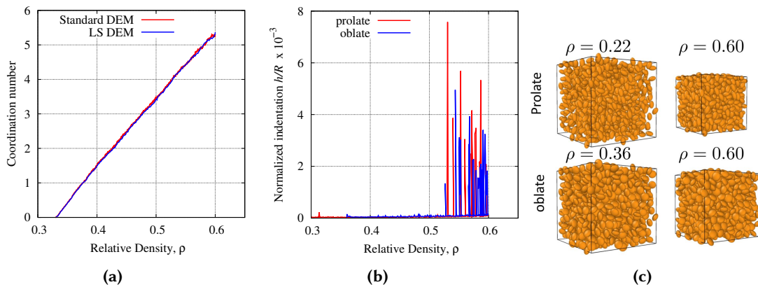
Figure 8: (a) Coordination number during jamming of spheres. (b) Mean indentation of ellipsoids as a function of relative density, \rho , during jamming. (c) Initial and final microstructures obtained.
