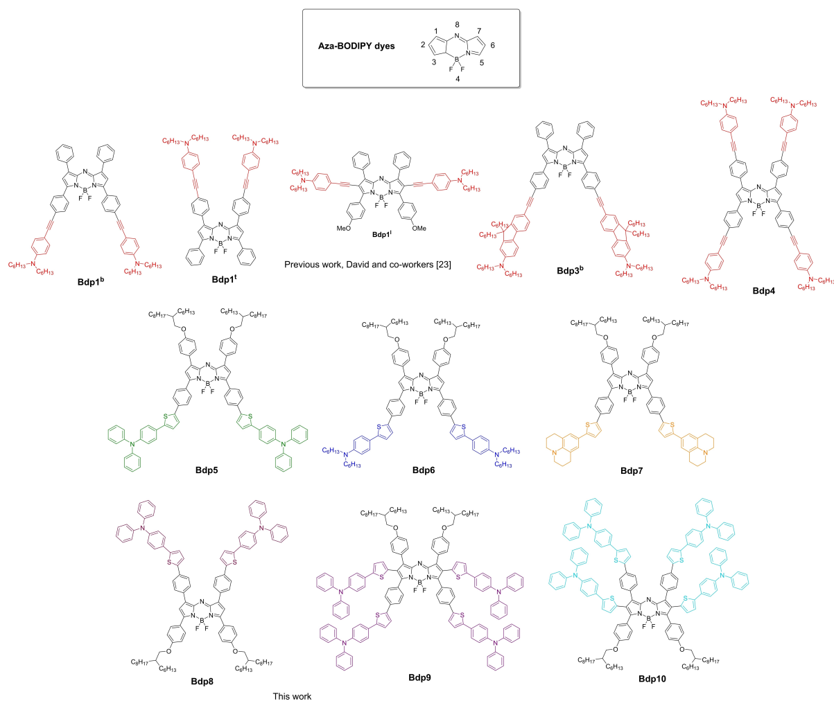
Figure 1. Structures of previously published aza-BODIPY dyes Bdp1 b , Bdp1 1 , Bdp1 1 , Bdp3 b , and Bdp4 designed for OPL at telecommunication wavelength and the new Bdp5-10 dyes investigated herein.
