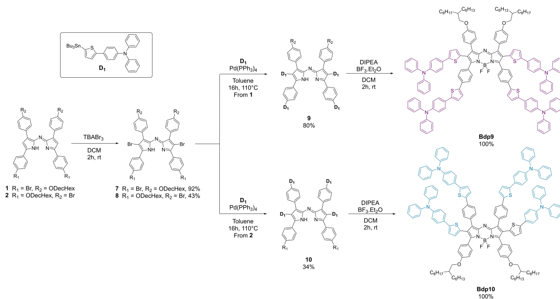
Scheme 2. Synthesis of the tetra-substituted aza-BODIPYs Bdp9 and Bdp10 .
