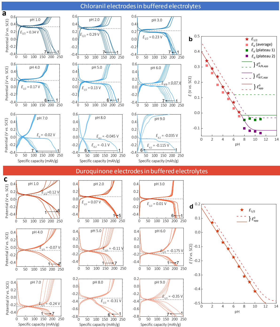
Figure 3. (a) GDC cycling profiles (the first 5 to 7 cycles are shown and the first cycle is highlighted in bold) of Ketjenblack EC-300J carbon-based chloranil electrodes (rate: 0.5 \text{ mA/cm}^2 ) in a set of buffered electrolytes at different pHs (the pH values are indicated on the graphs). (b) Average discharge potentials ( E_d ) of the single (red solid squares) or two plateaus (green and purple solid squares) extracted from the first galvanostatic discharges as a function of pH. The red solid stars correspond to the E_{1/2} extracted from the GDC cycles as a function of pH. The dashed red, green and purple curves are the theoretical E -pH plot of chloranil in homogeneous solution (same plots than in Figure 1c), while the solid green, purple and red curves are the best fits of eqs. 5, 6 and 9, respectively, to the experimental data using: \text{p}K_{a,3} = 9.0 , \text{p}K_{a,6} = 7.0 , E_1^0 = -0.014 \text{ V} and E_2^0 = -0.115 \text{ V} . (c) GDC cycling profiles (the first 5 to 7 cycles are shown and the first cycle is highlighted in bold) of Ketjenblack EC-300J carbon-based duroquinone electrodes (rate: 0.5 \text{ mA/cm}^2 ) in a set of buffered electrolytes at different pHs (the pH values are indicated on the graphs). (d) (red stars) Average discharge/charge plateau potential (or E_{1/2} ) extracted from the GDC cycles in c as a function of pH. The dashed red curve is the theoretical E_{app}^0 -pH plot of duroquinone in homogeneous solution (same plot than in Figure 1g), and the solid red line is the same as the dashed red line but vertically offset by -50 mV.
