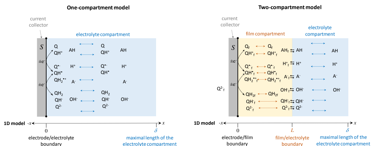
Scheme S1. Schematic representation of (left) the semi-infinite one-compartment 1D model and (right) finite/semi-infinite two-compartment 1D model.
