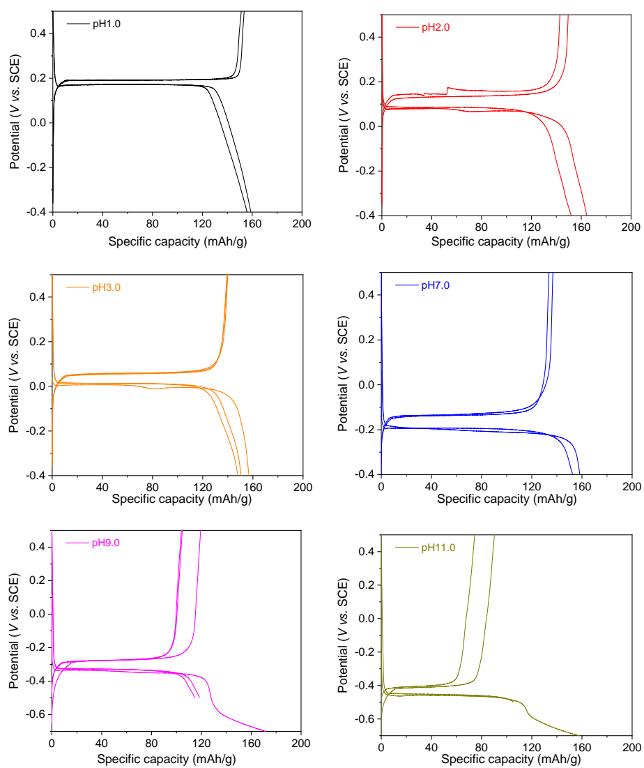
Figure S5. GDC cycling profiles (the first few cycles are shown) of Super P ® carbon-based duroquinone electrodes (rate: 0.5 mA/cm 2 ) in a set of buffered electrolytes at different pHs (the pH values are indicated on the graphs).
