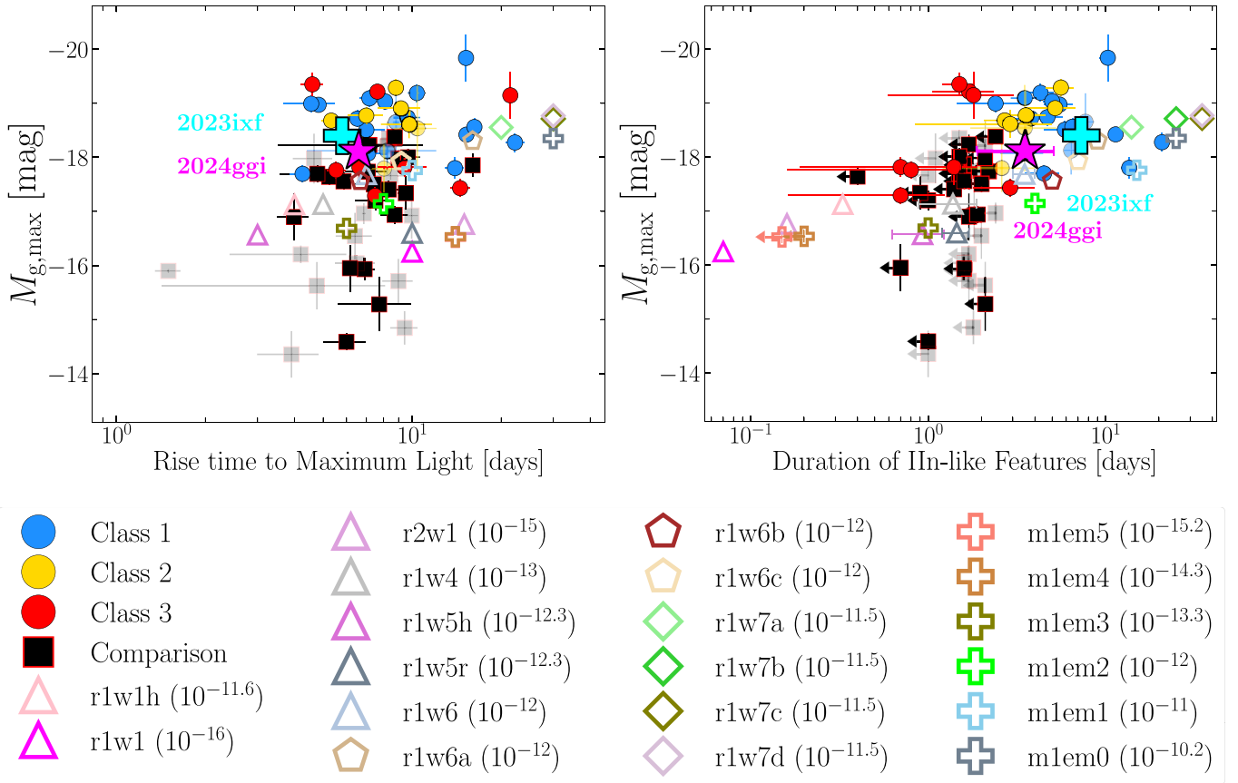
Figure 4. Peak g -band absolute magnitude vs. rise time (left) and duration of IIn-like features (right). Gold and silver samples are shown as blue, yellow, and red circles and the comparison sample is shown as black squares. Solid colored points represent the subsample of objects at D > 40 Mpc. Parameters from the CMFGEN model grid (Section 3.3) are plotted as colored stars, polygons, diamonds, and plus signs for CSM at 10^{14} cm (with density in units of g\text{ cm}^{-3} ) for each model displayed in parentheses. SNe 2024ggi and 2023ixf are shown as a magenta star and a cyan cross, respectively.
