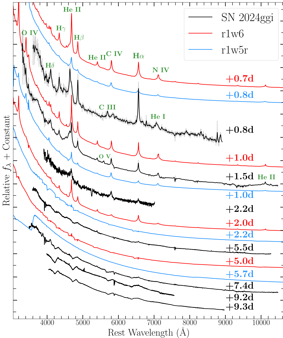
Figure 2. Early-time optical spectral series of SN 2024ggi (black) together with r1w6 (red) and r1w5r (blue) models from Dessart et al. (2017). The r1w6 and r1w5r models are characterized by wind mass-loss rates of \dot{M} = (0.5\text{--}1) \times 10^{-2} M_{\odot} \text{ yr}^{-1} that extend to a CSM radius of R_{\text{CSM}} = (2\text{--}5) \times 10^{14} cm. The model spectra have been smoothed with a Gaussian kernel to match the spectral resolution of the data. Line identifications are shown in green. The appearance of He II, C IV, N IV/V, and O V after the \delta t = +0.8 day spectrum indicates a rise in ionization and temperature in SN 2024ggi as the breakout pulse and the subsequent continuous release of radiation from the shock diffuses through the CSM.
