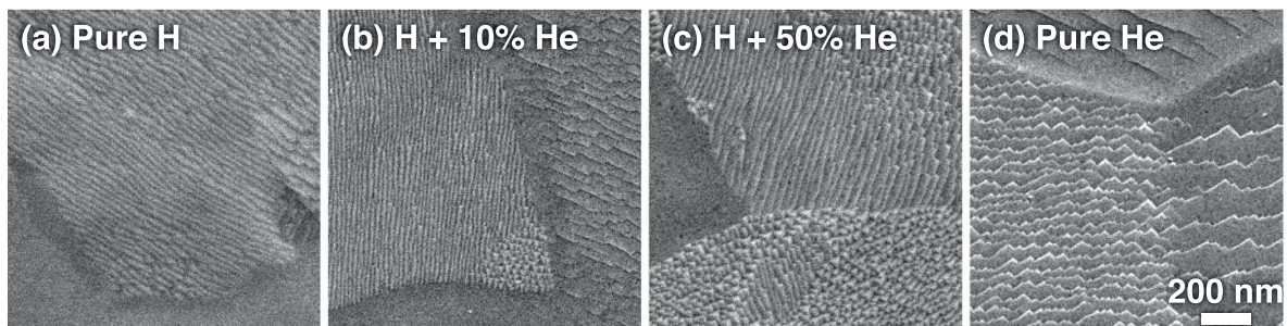
Figure 2. SEM images of (a) pure hydrogen plasma, (b) 10% helium mixed hydrogen plasma, (c) 50% helium mixed hydrogen plasma and (d) pure helium plasma exposed tungsten surface at a fluence of 1 \times 10^{26} \text{ m}^{-2} .
