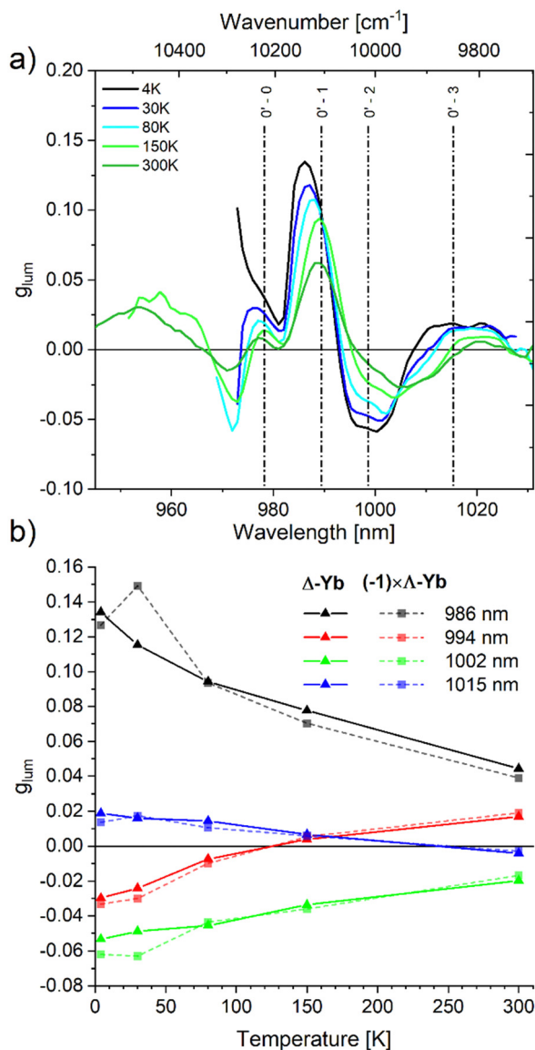
Fig. 5 (a) Variations of the emission dissymmetry factor, g_{lum} , of \Delta\text{-Yb} over its emission range at different temperatures (cut-off at 5% of the emission maximum for each temperature to discard erratic values at low intensities) with previously determined transitions energies from the 0' excited sublevel (Fig. 2a) (b) variation of dissymmetry factors with temperature at selected wavelengths (opposite-sign g_{lum} values are plotted for \Delta\text{-Yb} ).
