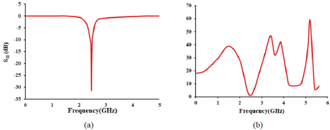
Figure 5. (a) Characteristics of reflection coefficient and (b) VSWR curve of meander antenna with partial ground
