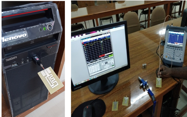
Figure 14. Measurement set up of proposed meander antenna with \lambda/5 dipole
