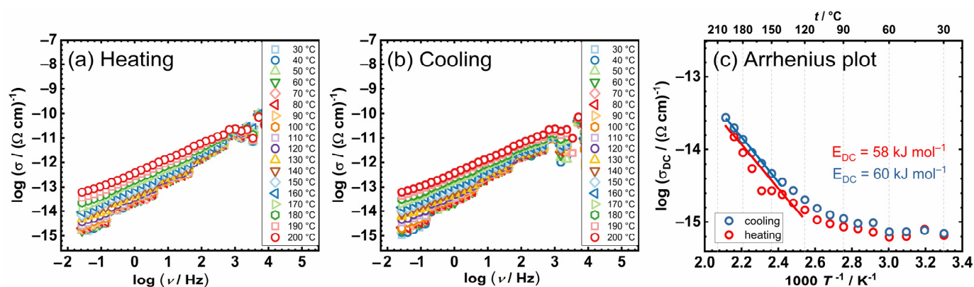
Figure 4. Conductivity spectra for [\text{MoO}_2(\text{L})(\text{MeOH})] (1) in (a) heating and (b) cooling runs, and (c) Arrhenius plot—temperature dependence of DC conductivity ( \log(\sigma_{\text{DC}}) vs. 1000/T ) for both runs (red circle—heating, blue circle—cooling).
