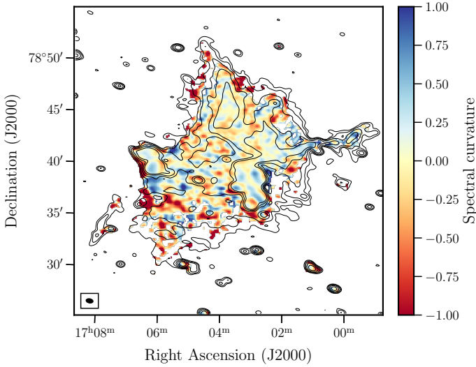
Fig. 8. Spectral index curvature map of Abell 2256, calculated as \alpha_{46\text{MHz}} - \alpha_{23\text{MHz}} - \alpha_{144\text{MHz}} , where both spectral index maps are made with a common resolution of 39'' \times 24'' . Blue regions indicate spectral steepening towards higher frequencies and red regions indicate flattening at higher frequencies. The background contours show the 144 MHz intensity smoothed to the same resolution.
