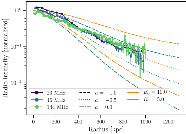
Fig. 13. Observed (points) and modelled (lines) radio halo synchrotron intensity profiles in Abell 2256. The parameter B_0 denotes the central magnetic field strength, and a the proportionality between cosmic ray energy density and thermal energy density. The details of the models are explained in Sect. 4.1.
