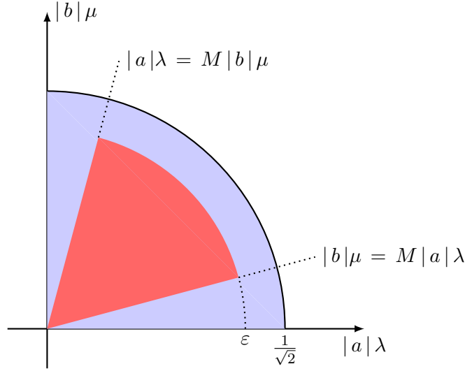
Figure 3.2: An illustration of admissible CFL parameters. The red area corresponds to the CFL parameters for which Theorem 3.1 holds, the blue one to the optimal set of parameters (for which stability for the Cauchy problem holds).
