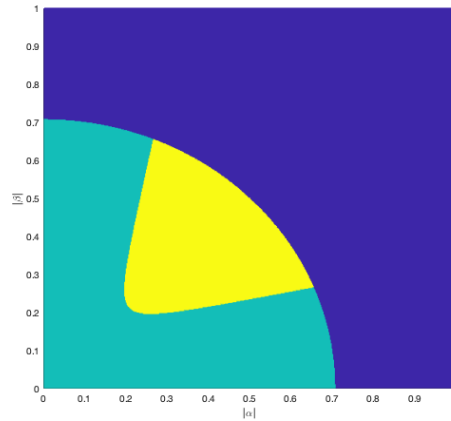
Figure 4.1: Negativity of the quadratic form associated with the corner contribution \mathcal{C} . In dark blue: the exterior of the ball. In yellow: the parameters (\lambda |a|, \mu |b|) for which (4.1) holds and the quadratic form is negative definite. In light blue: the parameters (\lambda |a|, \mu |b|) for which (4.1) holds and the quadratic form is not negative definite.
