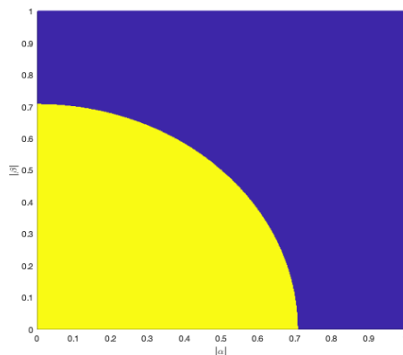
Figure 4.3: Negativity of the simplified boundary contribution \tilde{\mathcal{B}} . In dark blue: the exterior of the ball. In yellow: the parameters (\lambda |a|, \mu |b|) for which (4.1) holds and the quadratic form is negative definite. In light blue: the parameters (\lambda |a|, \mu |b|) for which (4.1) holds and the quadratic form is not negative definite.
