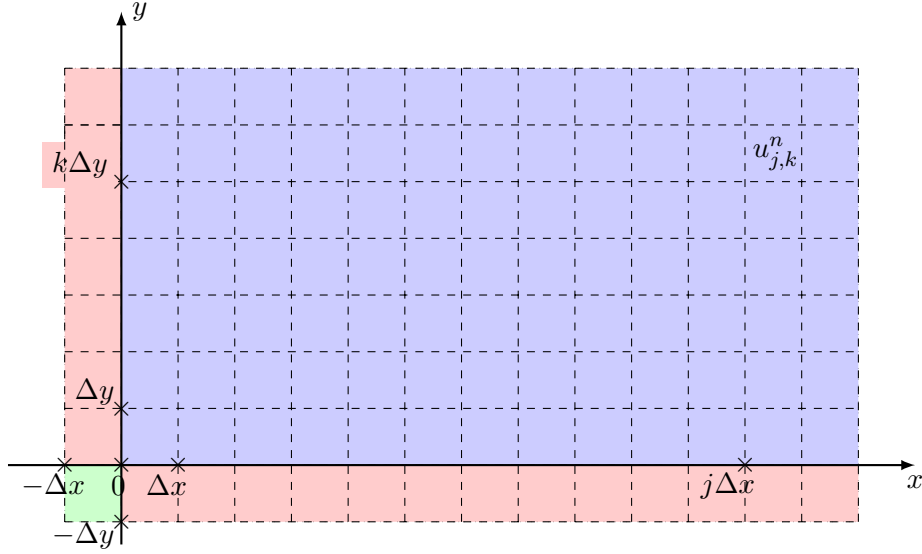
Figure 3.1: The spatial grid for the quarter-plane. Interior cells appear in blue, the boundary ghost cells appear in red and the corner ghost cell appears in green. The value u_{j,k}^n corresponds to the approximation in the cell [n \Delta t, (n + 1) \Delta t) \times [j \Delta x, (j + 1) \Delta x) \times [k \Delta y, (k + 1) \Delta y) .
