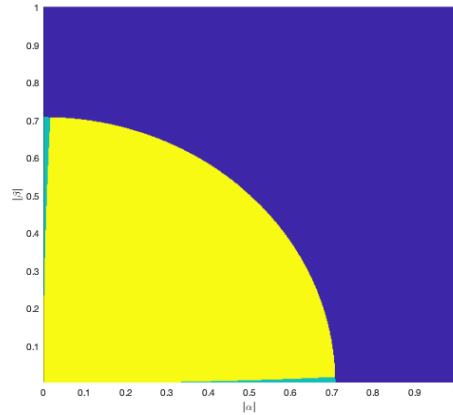
Figure 4.2: Negativity of the quadratic form associated with the reduced corner contribution \tilde{\mathcal{C}} . In dark blue: the exterior of the ball. In yellow: the parameters (\lambda|a|, \mu|b|) for which (4.1) holds and the quadratic form is negative definite. In light blue: the parameters (\lambda|a|, \mu|b|) for which (4.1) holds and the quadratic form is not negative definite.
