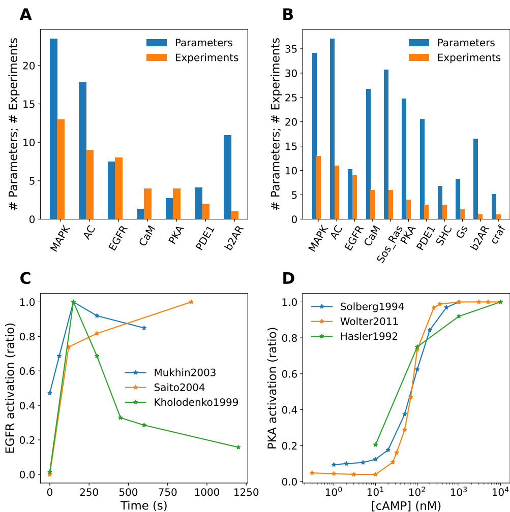
Figure 5. Features of experimental database. A, B: Number of parameters (blue) and number of experiments (orange) to constrain them, for different blocks in the model, sorted in order of decreasing number of experiments. In almost all cases the number of experiments falls well short of the number of parameters, that is, the model is underconstrained. A: Reduced (Hill/Tau) models. B: ODE (SBML) models. C, D: Experiments may be inconsistent. C: Three time-series experiments for EGFR activation following a pulse of EGF, normalized to maximal response. These experiments were performed on different cell lines and not surprisingly, the time-courses differ (56, 57, 58). D: Three dose-response experiments for PKA activation by cAMP. These experiments use purified preparations and despite somewhat different conditions the K_d is quite similar (59, 60, 61).
