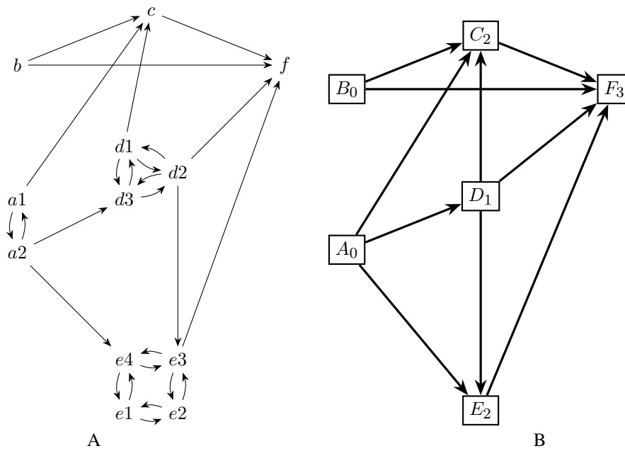
Figure 1. Interaction and quotient graphs used for the hierarchical decomposition. A) The interaction graph is a directed graph whose nodes are biochemical species. One source species acts on a target species if there is a reaction consuming or producing the target, whose rate depends on the concentration of the source. The strongly connected components (SCC) are maximal sets of nodes such that there are paths connecting each node to any other node. This graph has six SCCs: A_0 = \{a_1, a_2\} , B_0 = \{b\} , D_1 = \{d_1, d_2, d_3\} , C_2 = \{c\} , E_2 = \{e_1, e_2, e_3, e_4\} , F_3 = \{f\} . B) The quotient graph is an acyclic directed graph, whose vertices are the SCC of the interaction graph. Two SCC are connected in the quotient graph if there is a species in one connected to a species in the other. The hierarchy level of a block (SCC) is the length of the longest path in the quotient graph, connecting a root to the block. In this example, blocks A, B are roots and have level 0, block D has level 1, blocks C, E have level 2 and F have level 3.
