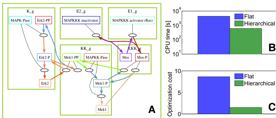
Figure 6. Optimization of the reduced MAPK model. A) Blocks in the reduced model; a three level nested hierarchy is defined as follows: level 1 (E1_g, E2_g, KKK_g), level2 (E1_g, E2_g, KKK_g, KK_g), level3 (E1_g, E2_g, KKK_g, KK_g, K_g). B,C) Performance of flat and hierarchical optimization.
