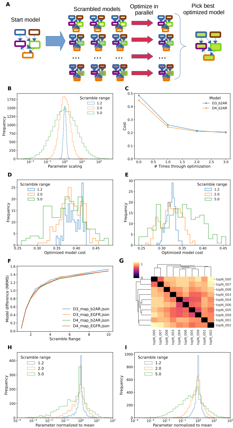
Figure 9. InitScram method. A. Schematic of method. B. log-normal distribution of parameter scaling from reference values for scrambleRange (SR) of 1.2, 2.0, and 5.0. C. Improvement of fit over successive optimizations. A second optimization produces a small improvement, and little improvement results from a third round. D. Cost distributions for three values of SR, D3 b2AR model. Note that the peaks are similar but the widths greater for larger SR, hence there are parameter sets with smaller costs (left tail of distribution) for large SR. E. Cost distributions for 3 values of SR, D4 b2AR model. Here the peaks of the cost distribution moves to the left with smaller SR. F. Mapping between parameter scrambling range and NRMS metric for similarity of models shows that this is independent of model. G. Model optimization cost cluster-map for top 10 optimized D4 b2AR models. H. Distribution of parameter scaling for optimized D3-b2AR models, normalized to mean of respective parameter for the best 10 models from that run. The optimized parameters converge very closely to the best 10 means. I. Distribution of parameter scaling for optimized D4-b2AR models. Here the tails of the distributions are somewhat wider, but there is still a narrow peak around 1.0 showing convergence from different start points. Note that peaks are narrower than the initial parameter ranges from panel B.
