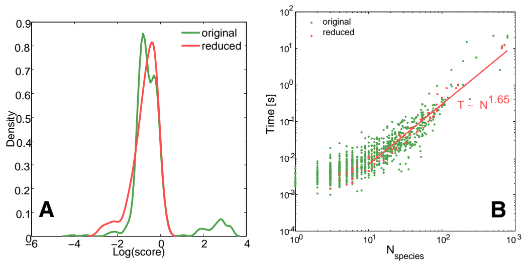
Figure 6: Benchmarking the hierarchical decomposition algorithm using 1058 models from the Biomodels repository [26]. A) The probability density of the decomposition score shows that QSS reduction of models with enzymes shared between multiple substrates improves the score. B) The algorithm has sub-quadratic complexity in the average.
