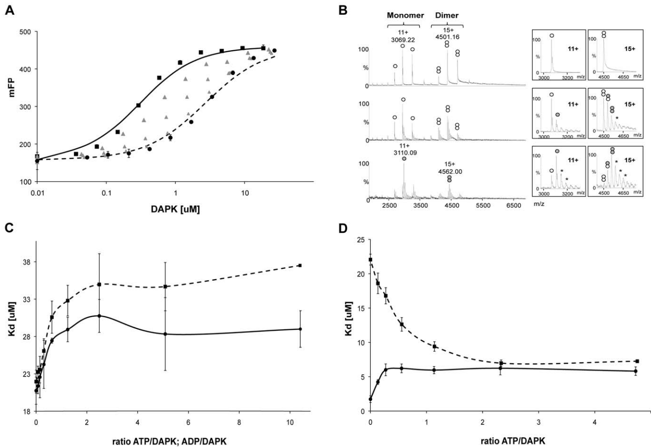
Figure 4. ATP/ADP binding to the catalytic domain of DAPK. A) Binding of the fluorescently tagged ATP (Atto-495-ATP) to the catalytic domain of DAPKwt. mFP corresponds to the polarization degree of the fluorescent probe \times 10^3 . One binding curve corresponds to a constant concentration of \text{NH}_4\text{Ac} , pH 8.8: \bullet 5 mM; from \blacktriangle to \blacktriangle 25, 50 and 100 mM, \blacksquare 250 mM. The binding curve of ATP shifts towards the left when the monomeric form is induced by higher \text{NH}_4\text{Ac} concentrations. B) Noncovalent mass spectrometry analysis of DAPKwt at 5 \mu\text{M} in 50 mM \text{NH}_4\text{Ac} buffer at pH 8.8 either alone (top) or in the presence of 25 \mu\text{M} ADP-Mg (middle) or 100 \mu\text{M} ADP-Mg (bottom). Inserts correspond to enlargements of 11+ and 15+ charge states of monomeric and dimeric DAPKwt, respectively. (O), (●), (⊗), (⊗) and (⊗) are related to 1:0, 1:1, 2:0, 2:1 and 2:2 DAPKwt: ADP-Mg complexes respectively. * represent non-specific ADP-Mg adducts. C) Fitted K_d values of the fluorescent probe as a function of ATP/DAPKdel (—●—) and ADP/DAPKdel (---■---) ratios. D) DAPKwt is assayed under conditions favoring monomers (—●— 250 mM \text{NH}_4\text{Ac} , pH 8.8) or dimers (---■--- 5 mM \text{NH}_4\text{Ac} , pH 8.8). doi:10.1371/journal.pone.0014120.g004
