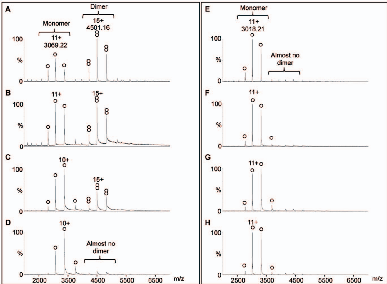
Figure 1. Noncovalent mass spectrometry analysis of (A–D) DAPKwt and (E–H) DAPKdel. Proteins were diluted to 5 μM in NH 4 Ac buffer at (A, E) 5 mM, (B, F) 50 mM, (C, G) 120 mM and (D, H) 250 mM. (○) and (⊠) are related to monomeric and dimeric DAPK, respectively. doi:10.1371/journal.pone.0014120.g001
