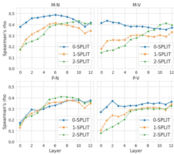
Figure 2: BERT AVG results by layer and split-type on every SPLIT-SIM subset.
