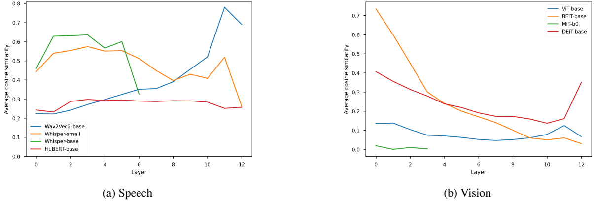
Figure 3: Average cosine-similarity between hidden representations across layers for Speech and Vision modalities. We observe that across both modalities, several models display significant levels of anisotropy.
