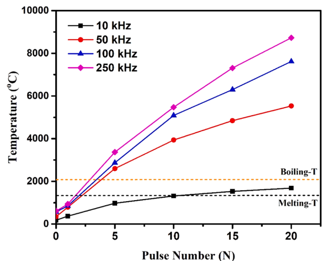
Fig. 9. The evolution of the calculated temperature with respect to the pulse number at various repetition rates, at a radial position of ( r = 0 \mu\text{m} ) from the center of the laser beam. The dashed lines indicates the melting and boiling temperatures.
