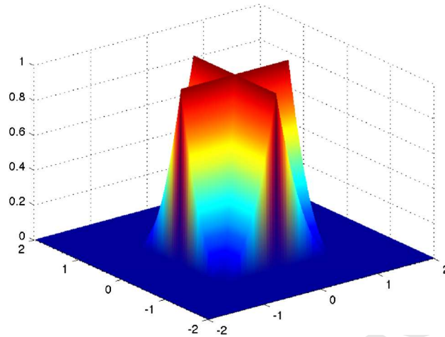
Fig. 4. \pi^\Delta(x, y) = (1 - \min(|x|, |y|))^2 .
