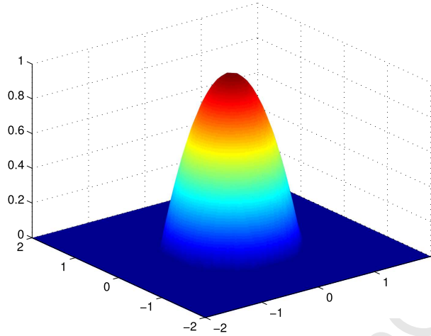
Fig. 2. \pi^\Delta(x) = \max(0, 1 - \|x\|^2) .
