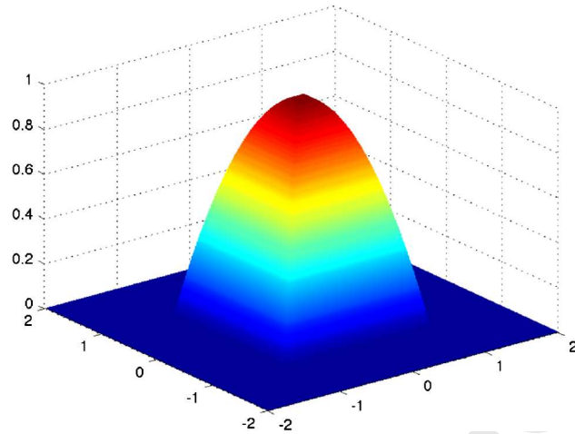
Fig. 3. \pi^\Delta(x, y) = 1 - \max(|x|, |y|)^2 .
