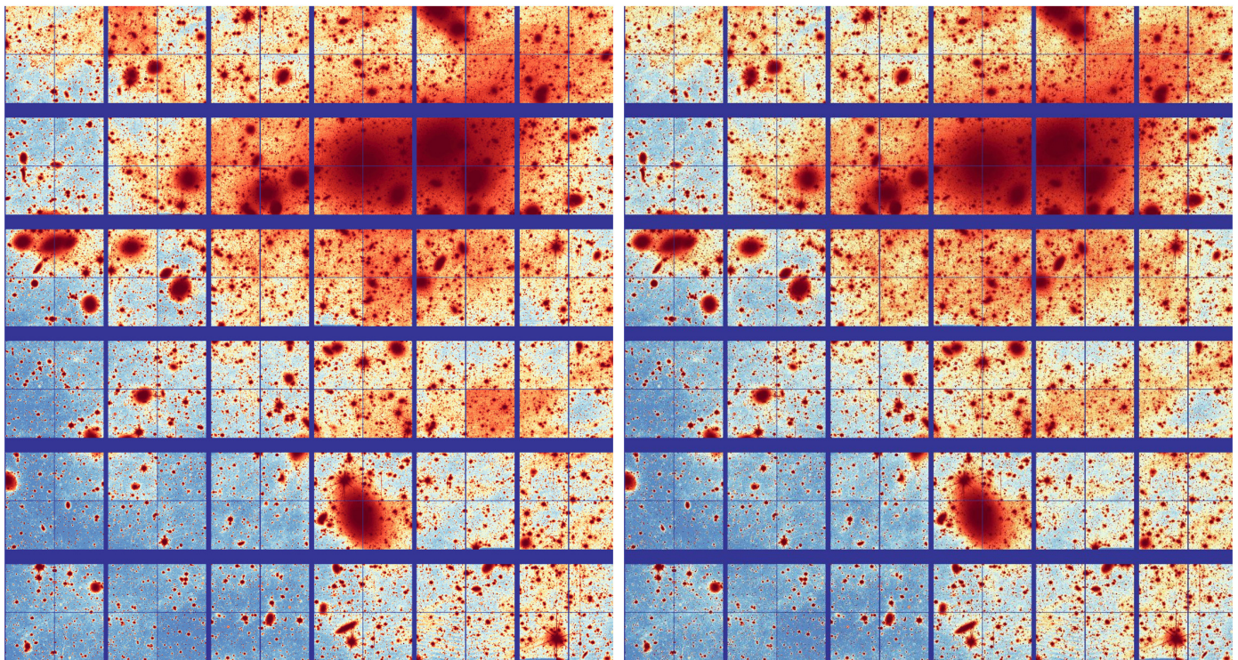
Fig. 5. Left: VIS image of the Perseus cluster following the ERO mask, overscan, bias, flat-field, and deepCR corrections reveals a checkerboard pattern in a small number of quadrants. The effect is 2% of the background for the two most affected quadrants (if left uncorrected this would leave residuals at the 27 to 28th mag arcsec -2 level). Right: final image, after applying a low-flux nonlinearity correction to approximately 30 quadrants. This now displays uniform flatness of the background across all borders—both between detectors and within quadrants—indicating reliable photometry for extended emission such as galaxy stellar halos, intra-cluster light, and Galactic cirrus, as showcased here. The limiting surface brightness of these single frames exceeds 29 mag arcsec -2 throughout the entire FoV (direct detection of faint contrasts at the 10'' scale).
