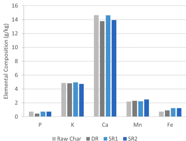
Fig. 10. Summary of the main inorganic elements in raw and spent chars samples. (colored).
