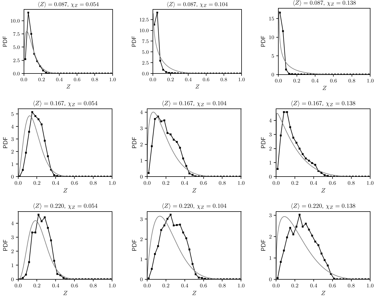
Fig. E.21. Conditional probability density function P(Z|\langle Z \rangle, \chi_Z) for different values of \langle Z \rangle and \chi_Z (■); presumed Beta distribution (—) function, F_{F_d^{-1}} = 0.486 .
