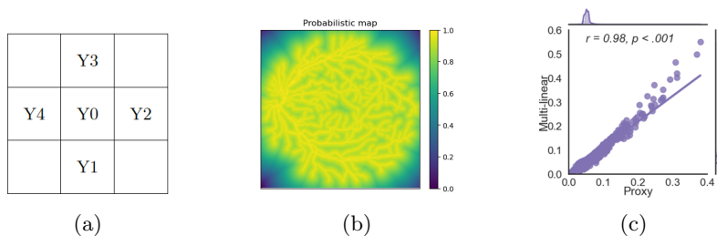
Fig. 1: (a) Definition of the 4 + 1 neighborhood variables; (b) Probabilistic map created from a binary retinal blood vessel; (c) Match between the output of 2D thinning operators based on multilinear vs proxy polynomials.
