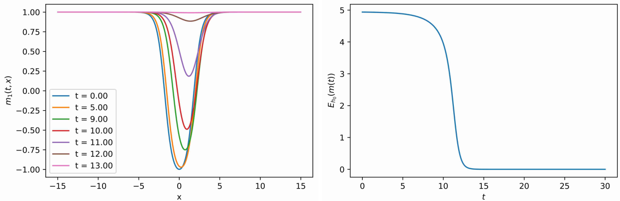
Figure 3: Left: Plot of m_1(t) for several time between 0 and 13. Right: Evolution of the modified energy E_{h_0}(m(t)) . The initial data is a perturbation of the stationary solution w_{h_0} with h_0 = 0.1 , as depicted in Section 5.2.
