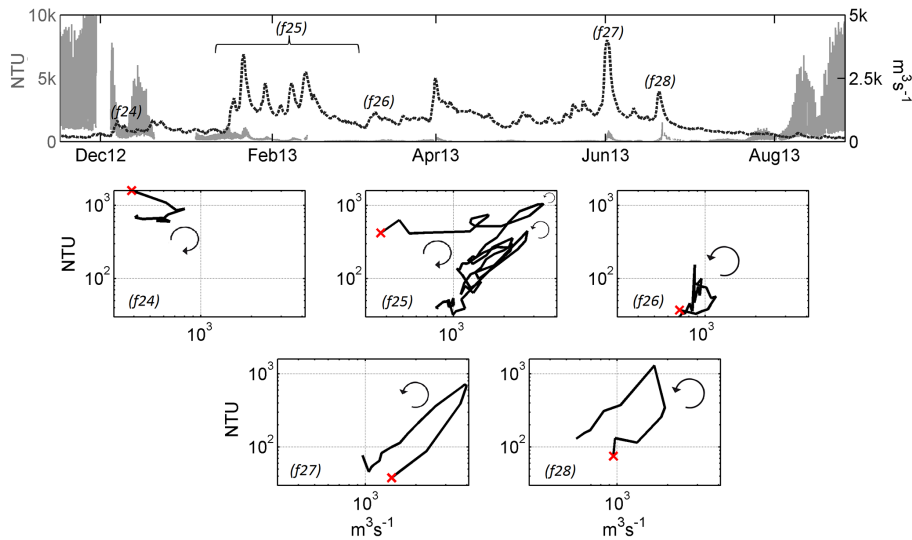
Figure 7. Relationship between Garonne discharge and turbidity at Bordeaux, and corresponding hysteresis patterns for the successive floods occurring since the downstream flushing, in December 2012, and the following upstream migration, in August 2013, of the TMZ; f plus a number refers to the flood events according to Fig. 3 and Table 1.
