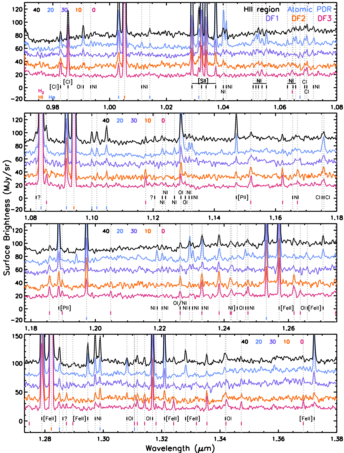
Fig. B.1. Spectral inventory of the five template spectra. Spectra are offset by the numbers given at the top of the panel. Areas susceptible to the wavelength gap are shown in light grey. The colour coding is labelled in the top panel.
