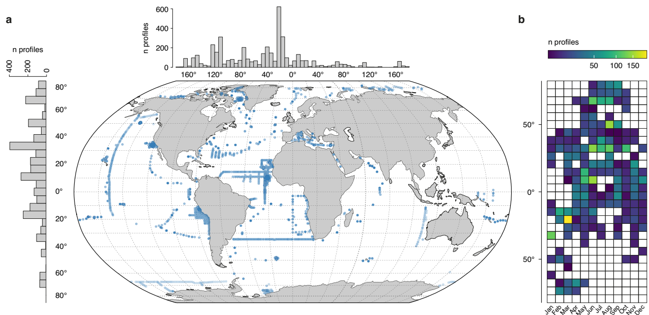
Fig. 1 | Spatial and temporal coverage of the 4252 vertical in situ profiles. a Geographic location of Underwater Vision Profiler 5 profiles used in this study. Left and top histograms show the latitudinal and longitudinal distribution of profiles along 3° bins. b Seasonal distribution of sampling points according to latitude.
