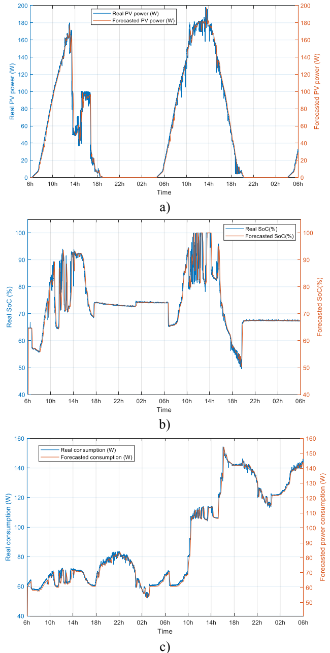
Fig. 5. a) Predictive and real PV generation, b) Predictive and real SoC, c) Predictive and real loads consumption
