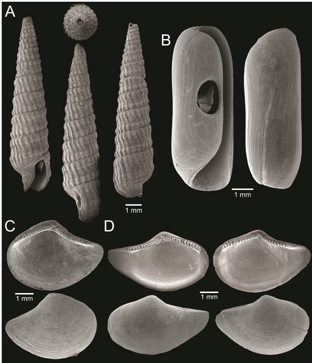
Figure 10. Gastropods and bivalves. A Duplicaria tricincta B Cylichna modesta C Jupiteria puellata D Saccella mauritiana .
