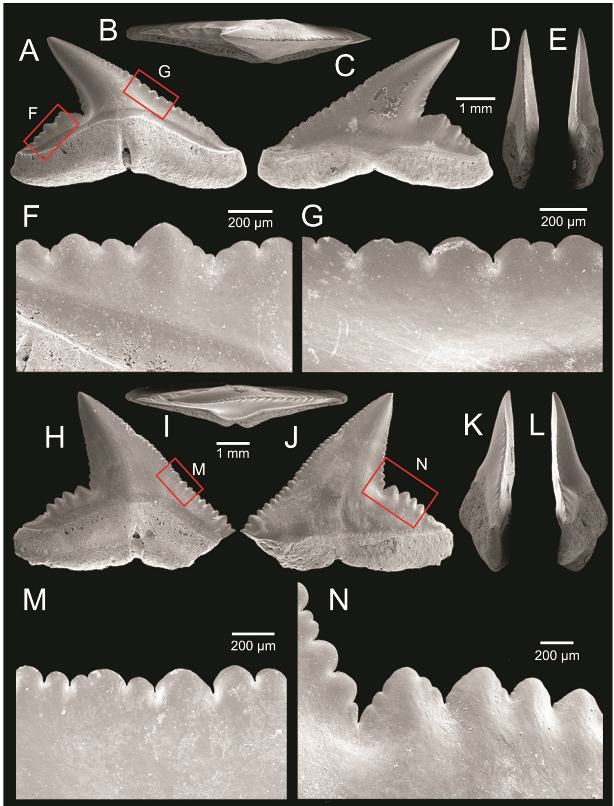
Figure 20. Carcharhinid shark teeth - Carcharhinus cf. sorrah A–G specimen CUF-NKNY-3.1 A lingual B apical C labial D mesial and E distal views F , G close-ups of the serration F on the distal heel and G on the middle part of the cusp mesial cutting-edge H–N specimen CUF-NKNY-3.2 H lingual I apical J labial K mesial and L distal views M close-up of the serration on the lower part of the mesial cutting-edge and N close-up of the serration between the heel and the base of the distal cutting edge.
