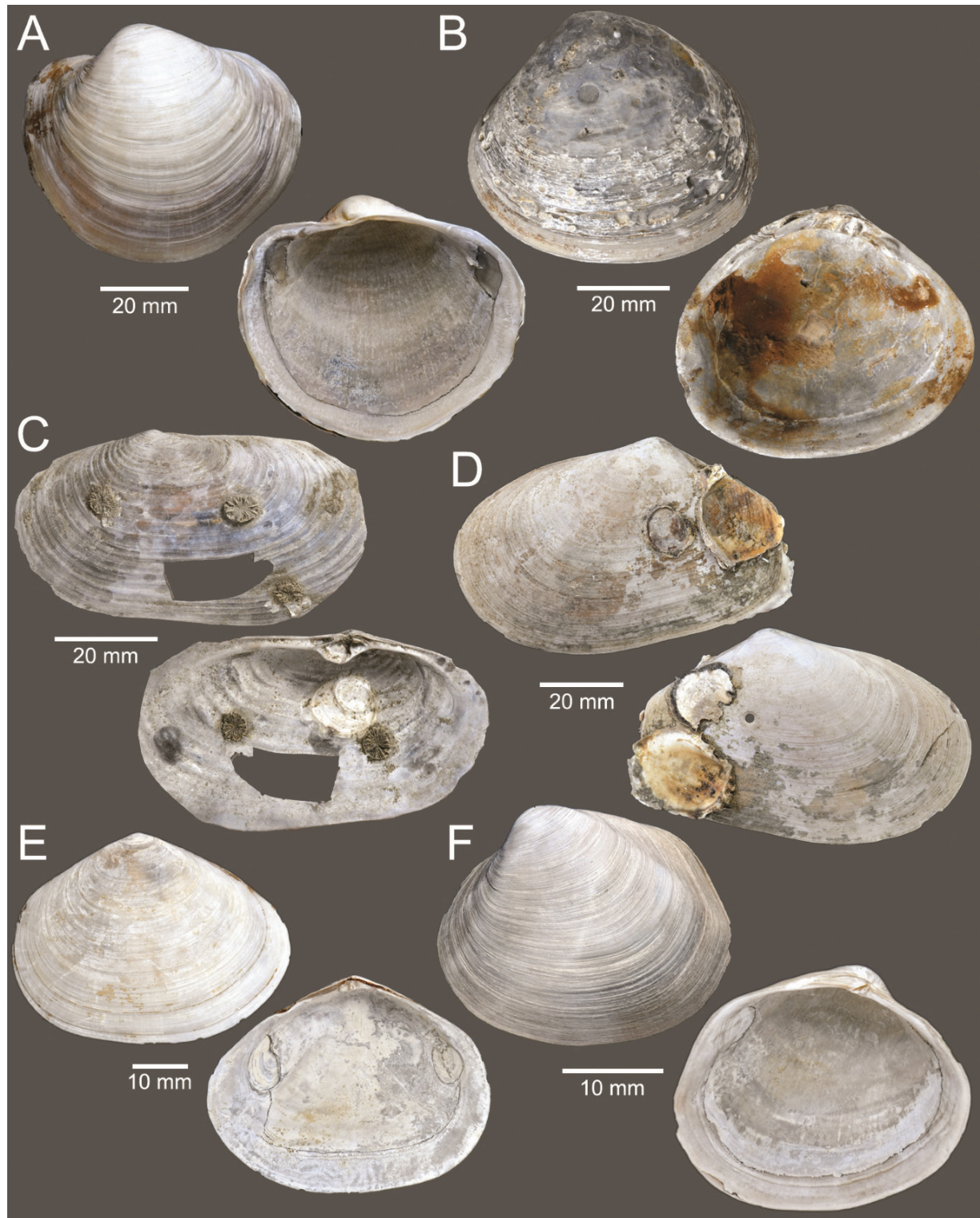
Figure 15. Bivalves A Pegophysema bialata B Geloina bengalensis C Lutraria complanata D Standella pellucida E Tellinides conspicuus F Joanniella oblonga .
