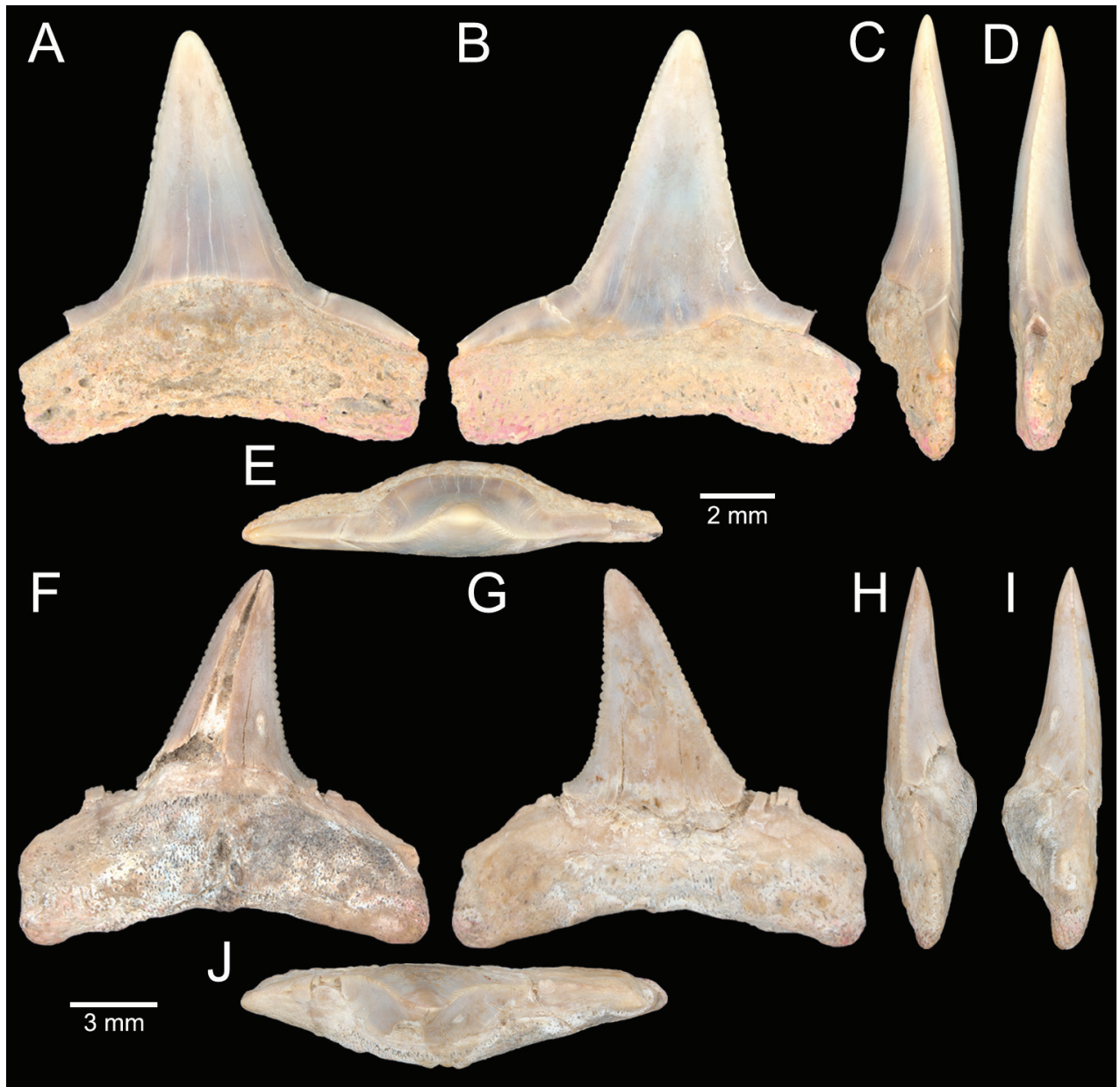
Figure 18. Carcharhinid shark teeth A–E Carcharhinus cf. amblyrhynchoides , specimen CUF-NKNY-S3-2 in A lingual B labial C mesial D distal and E apical views F–J Carcharhinus cf. amblyrhynchos , specimen CUF-NKNY-S3-10 in F lingual G labial H mesial I distal and J apical views.
