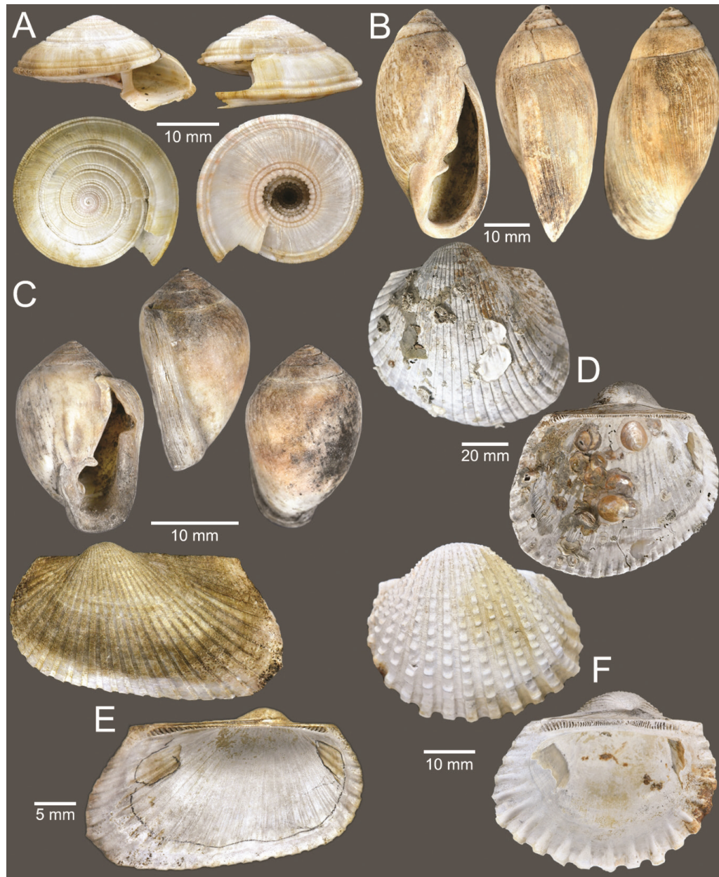
Figure 11. Gastropods and bivalves A Architectonica perdis B Ellobium aurisjudae C Cassidula nucleus D Anadara inaequalis E Anadara indica F Tegillarca granosa .
