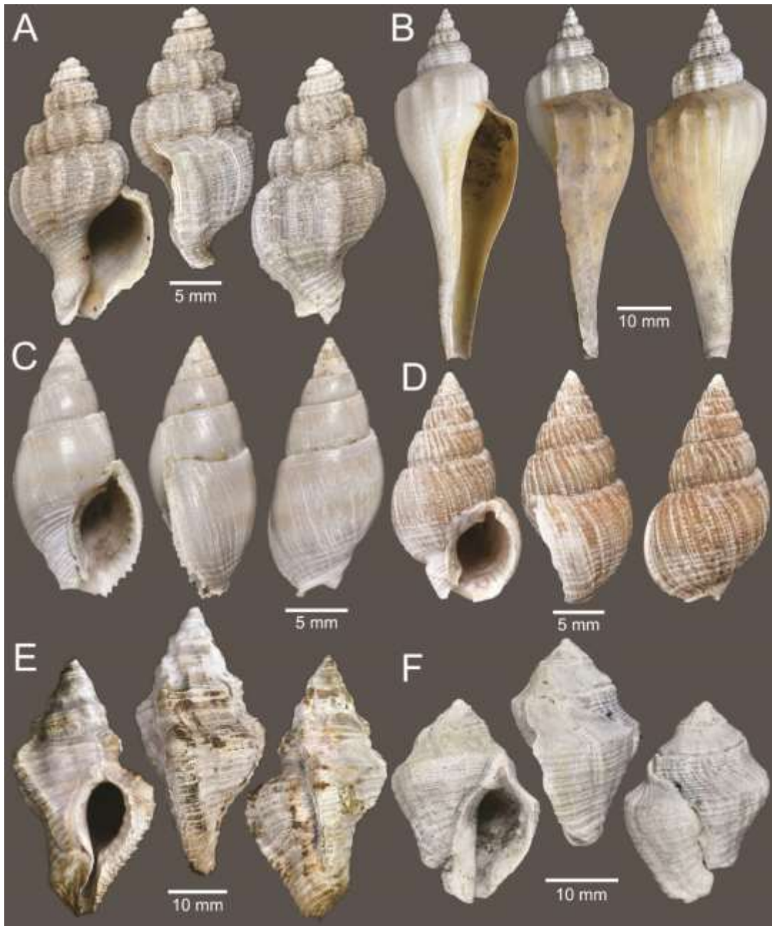
Fig. 7. Gastropods. A Pseudoneptunea varicosa B Brunneifusus ternatanus C Nassarius micans D Nassarius siquijorensis E Chicoreus capucinus F Indothais gradata .
