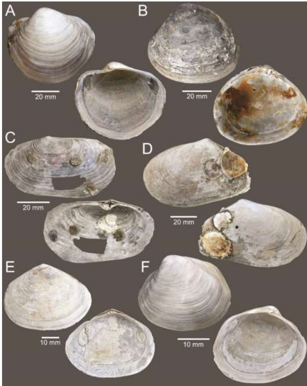
Fig. 15. Bivalves. A Pegophysema bialata B Geloina bengalensis C Lutraria complanata D Standella pellucida E Tellinides conspicuus F Joannisiella oblonga .
