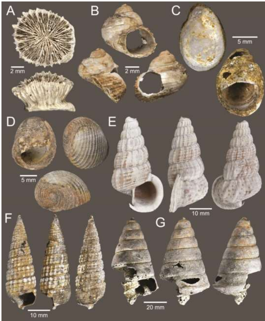
Fig. 5. Coral and gastropods. A Oulangia cf. stokesiana B Homalopoma cf. sangarense C Neripteron cf. violaceum D Nerita articulata E Cerithidea obtusa F Pirenella incisa G Telescopium telescopium .
