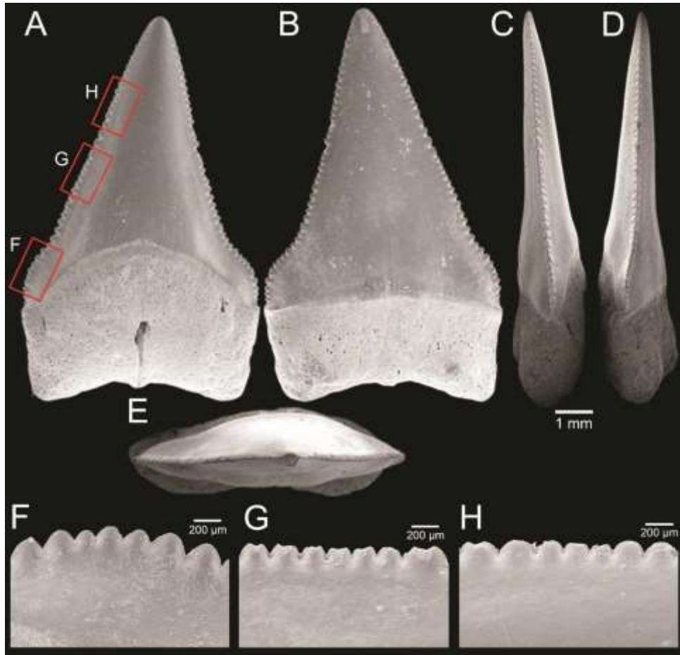
Fig. 24. Carcharhinid shark teeth - Glyphis sp. specimen CUF-NKNY-Q03, upper anterior tooth in A lingual B labial C mesial D distal and E apical views F–H close-ups of the serration F at the base, G in the middle and H in the upper part of the cusp mesial cutting-edge.
