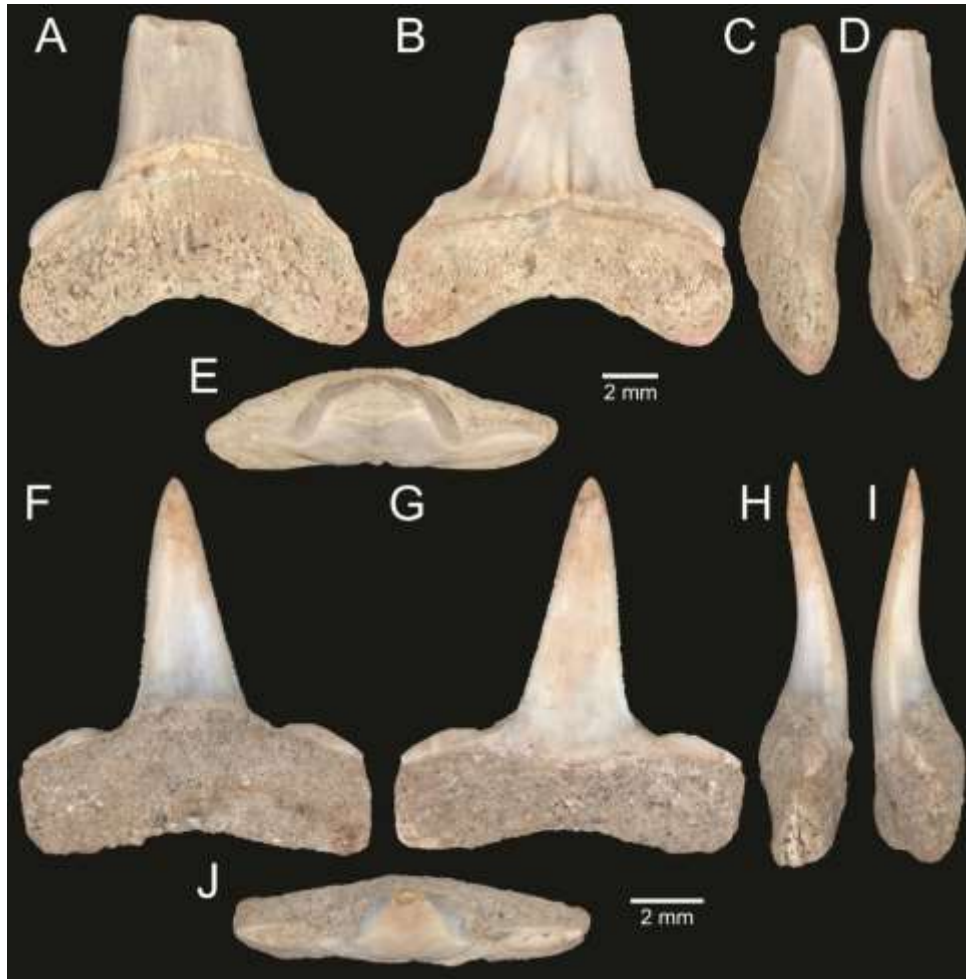
Fig. 27. Carcharhinid shark teeth - Glyphis sp. A–E specimen CUF-NKNY-S3-1, lower tooth in A lingual B labial C mesial D distal and E apical views F–J specimen CUF-NKNY-S3-6, lower tooth in F lingual G labial H mesial I distal and J apical views.
