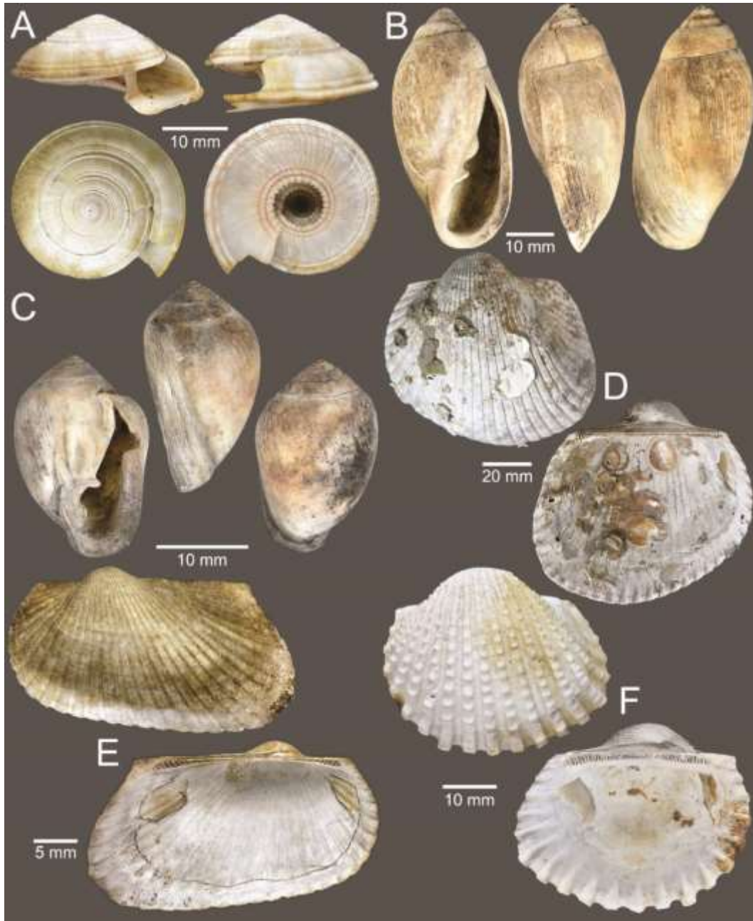
Fig. 11. Gastropods and bivalves. A Architectonica perdix B Ellobium aurisjudae C Cassidula nucleus D Anadara inaequalvis E Anadara indica F Tegillarca granosa .
