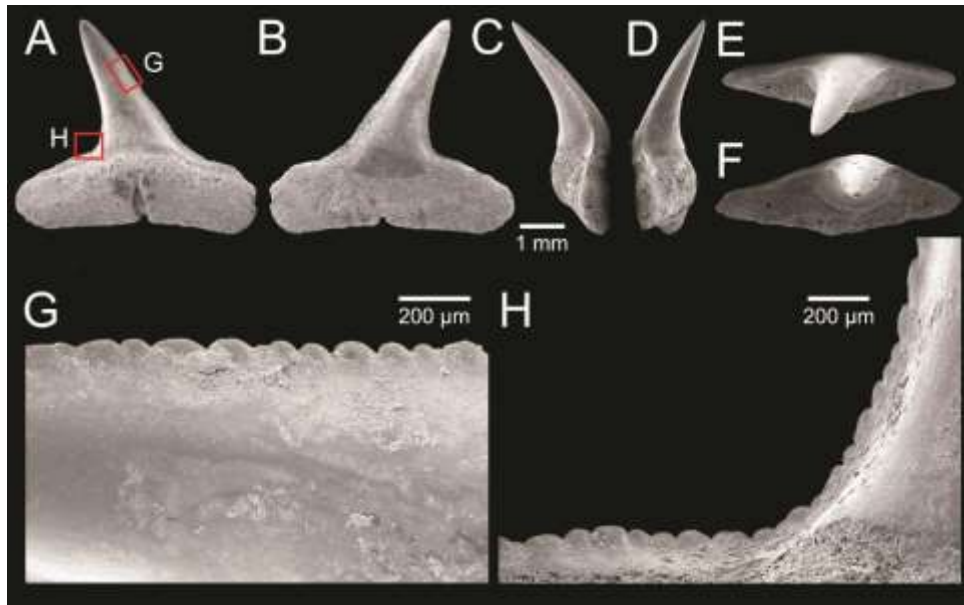
Fig. 22. Carcharhinid shark teeth - Carcharhinus sp. A–H specimen CUF-NKNY-S1 in A lingual B labial C mesial D distal and E, F apical views G, H close-ups on the serration G at mid-height of the cusp mesial cutting-edge and H at the level of the distal heel and base of the cusp.
