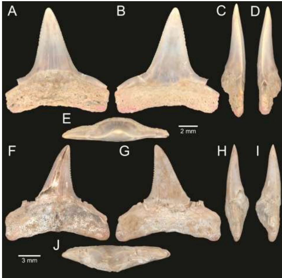
Fig. 18. Carcharhinid shark teeth. A–E Carcharhinus cf. amblyrhynchoides , specimen CUF-NKNY-S3-2 in A lingual B labial C mesial D distal and E apical views F–J Carcharhinus cf. amblyrhynchos , specimen CUF-NKNY-S3-10 in F lingual G labial H mesial I distal and J apical views.
