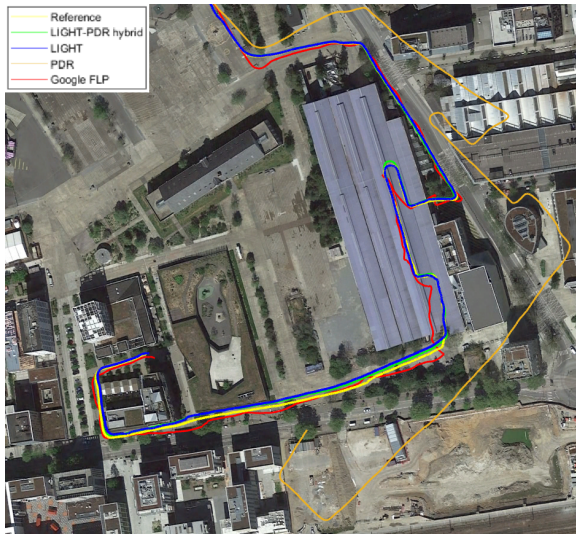
Fig. 21. Trajectories for Urban/shipyard dataset (green: LIGHT-PDR hybrid, blue: LIGHT-only, orange: PDR-only, yellow: reference, red: Google FLP) (Background satellite image source: Google Earth)
