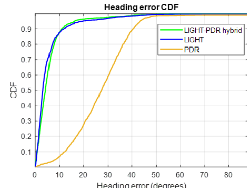
(b) Heading error CDF
