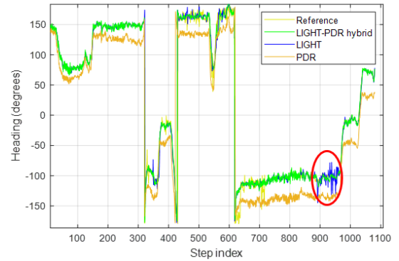
(a) Heading comparison
