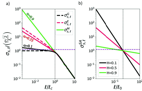
Figure 9. Standard deviation of local slopes as a function of length scale \ell over which it is defined for surfaces with following ACFs: (a) comparison of exponential and Gaussian ACFs as well as ACF of mounded surface ( \ell_0=35\mu\text{m}, \ell_c=25.6\mu\text{m}, \Lambda=220\mu\text{m}, \alpha=0.1;0.55;0.9 ); (b) ACF of self-affine surfaces with different values of Hurst exponent.
