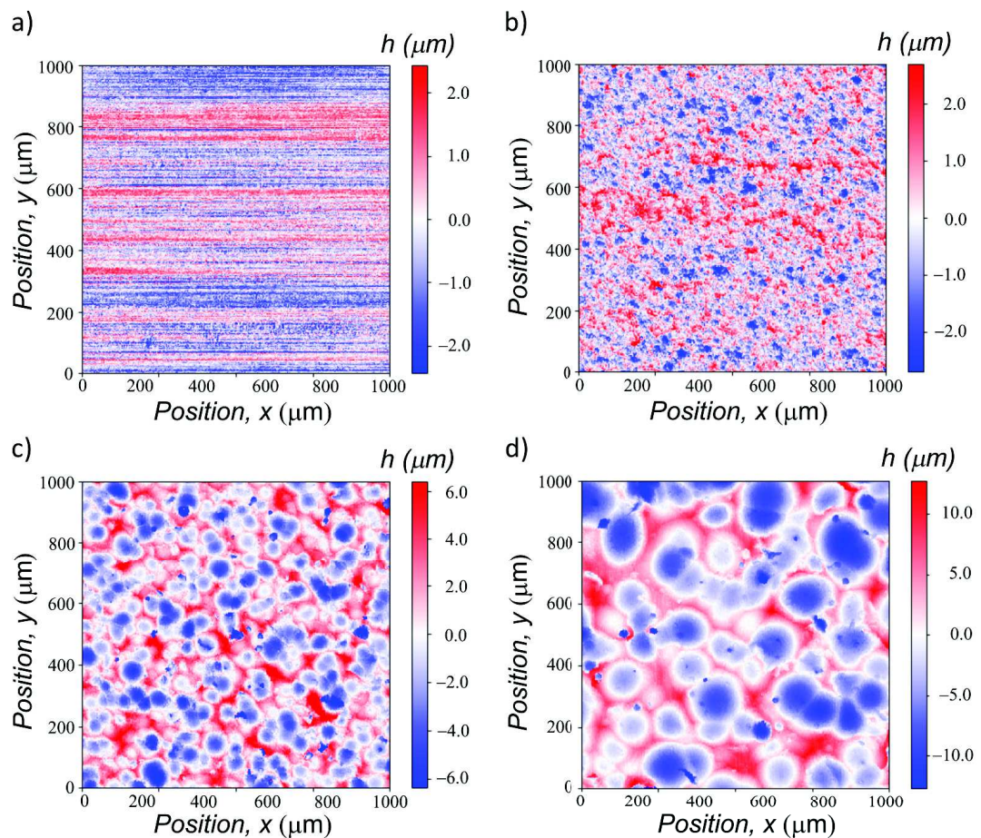
Figure 2. Contour plots of the 2D topography maps of the examined samples obtained from an optical profilometer: untreated sample (a), and samples blasted with small (b), medium (c) and large (d) beads. The dimensions of each map were 1 \times 1 \text{ mm}^2 and the lateral resolution was 2 \mu\text{m} . The color-scale gives the height in microns with respect to the mean surface ( z = 0 ) and the range of the color-scale is \pm 2.5\sigma for each sample.
