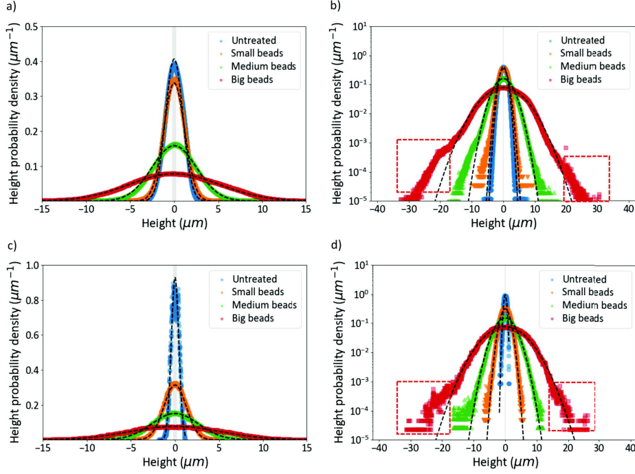
Figure 4. Height distribution of the four samples, obtained from measurements with (a,b) optical profilometer and (c,d) stylus profilometer plotted in linear (a,c) and logarithmic scale (b,d). Rectangles with dash red border indicate the data points impacted by measurement artifacts.
