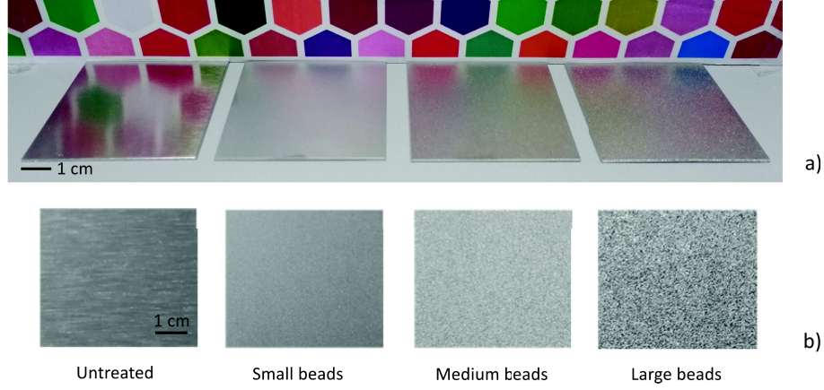
Figure 1. Photographs of the studied aluminum samples observed under D65 illumination: a) at grazing observation angle; b) at observation direction close to surface normal.
