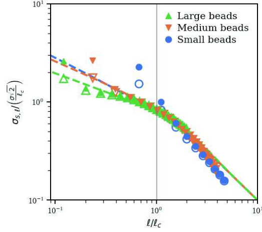
Figure 11. Standard deviation of slope distribution as a function of \ell , the size of fitted surface element. Variance is normalized by \sigma\sqrt{2}/\ell_c , while the size of surface element is normalized by \ell_c . Results obtained from paraboloid and plane fit are shown with filled and empty symbols respectively. Dash lines show theoretical curve on standard deviations of slope distribution from Eq. (23) for samples blasted with small (blue line), medium (green line) and large (red line) beads.
