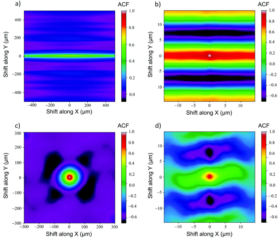
Figure 6. 2D-ACF of the untreated sample (a,b) and sample blasted with large beads (c,d) calculated from 2D height maps obtained with optical profilometer (a,c) and AFM (b,d).
