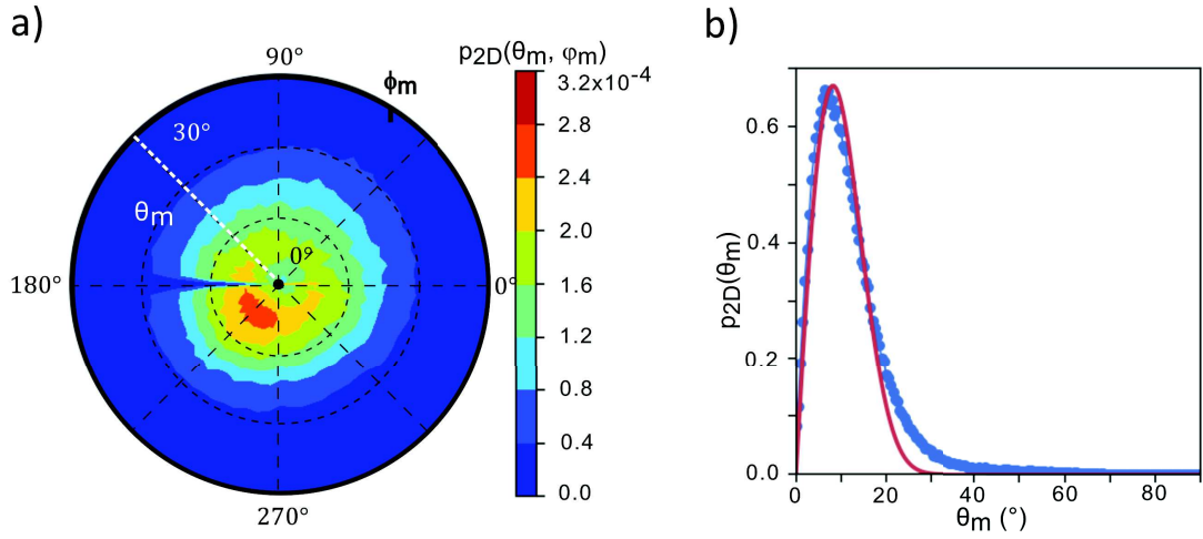
Figure 12. Slope angle distribution p_{2D}(\theta_m, \phi_m) of sample blasted with medium beads (a) and its radial average (b). Solid line on (b) shows the fit of data points with Eq. (28).
