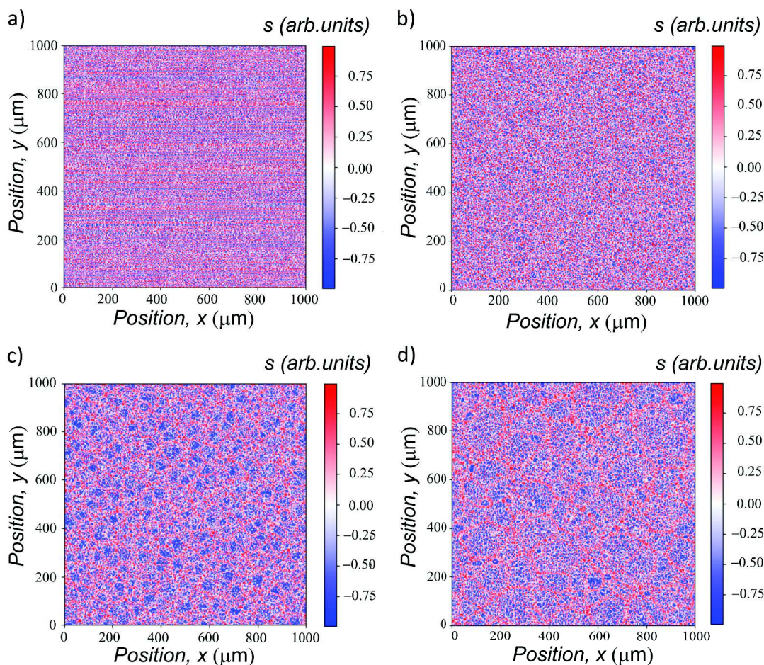
Figure 13. Shape index of the raw substrate (a) and surfaces blasted with small (b) medium (c) and large beads (d). The shape index progressively describes the local curvature from a spherical cup to a dome (respectively from -1 to 1).
