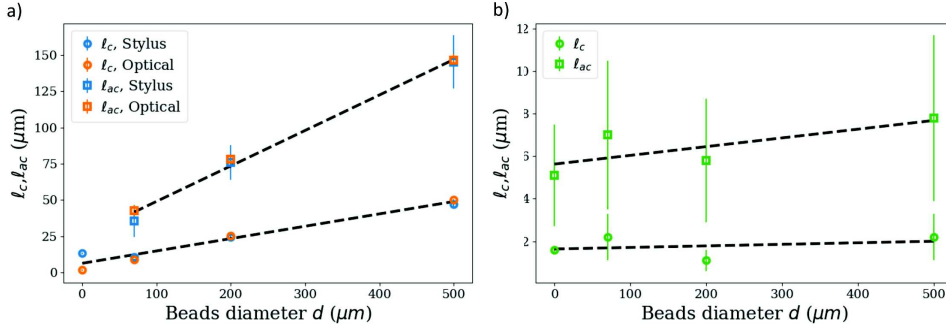
Figure 8. Correlation length \ell_c and anti-correlation length \ell_{ac} vs bead size obtained (a) at large scale by stylus and optical profilometry and (b) at small scale by AFM. The black dashed and continuous line show (a) an indicative linear trend and (b) an average behavior.
