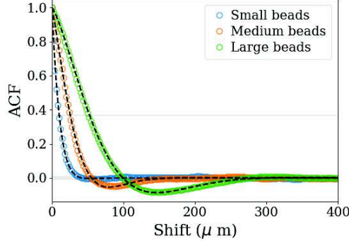
Figure 7. Radial ACFs of blasted aluminum samples, averaged over number of topography maps, obtained with optical profilometer.
