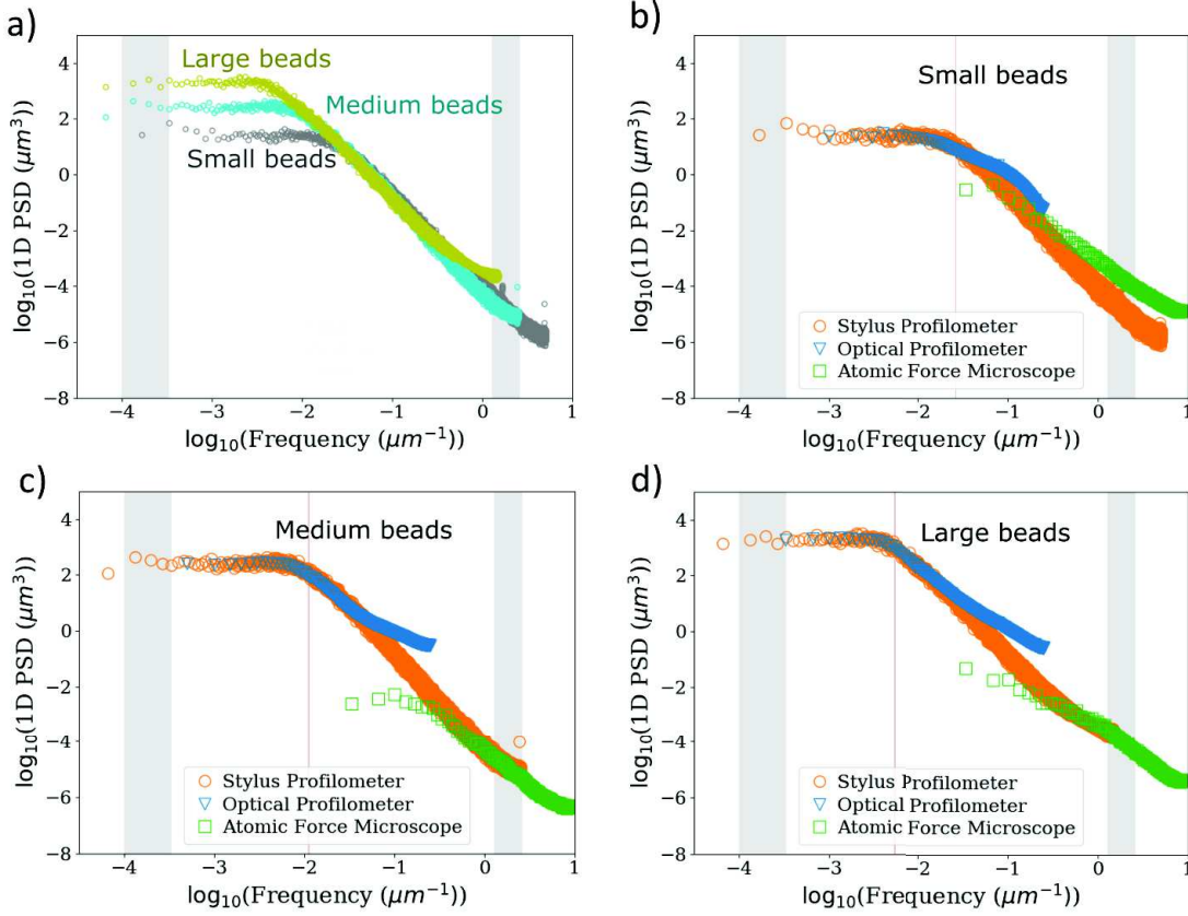
Figure 5. 1D-PSD curves of examined blasted samples: (a) superposition of 1D-PSD obtained with stylus profilometer for three blasted samples; and master curves for sample blasted with small (b), medium (c) and large beads (d). Each master curve contains 1D-PSDs calculated from data obtained with stylus profilometer (orange circles), optical profilometer (blue triangles) and AFM (green squares). Each plotted 1D-PSD curve is an average over the number of measurements (see table 1). PSDs of topography data from stylus profilometer are 1D-PSD by construction. PSDs based on data from optical profilometer and AFM are originally 2D-PSD and are converted to 1D-PSD (Eq. (15)), except for untreated sample which is represented by a cut of the 2D PSD in direction orthogonal to the grooves. The red vertical line on (b-d) indicates the breakpoint frequency of each sample. For the sake of readability, gray rectangles indicate typical lower and upper limits of spatial frequencies that participate into the optical response of the surface in scattering experiment in the visible spectral range under normal incidence. The lower limit is related to the size of beam used in light scattering experiment, 1/D_{spot} with D_{spot} \in [0.3; 1.0] cm. The upper limit (1 + \sin \theta_{inc})/\lambda is plotted for normal incidence and visible spectral range \lambda \in [480; 780] nm.
