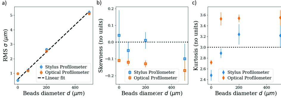
Figure 3. (a) RMS, (b) Skewness and (c) Kurtosis of the initial cold rolled aluminum surfaces and after blasting with particles of sizes.
