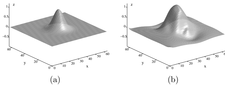
Figure 14: (a) Second starting shape and (b) associated result by M1 ( \lambda_{\text{int}} = 10 and \lambda_{\text{smo}} = 50 ).
