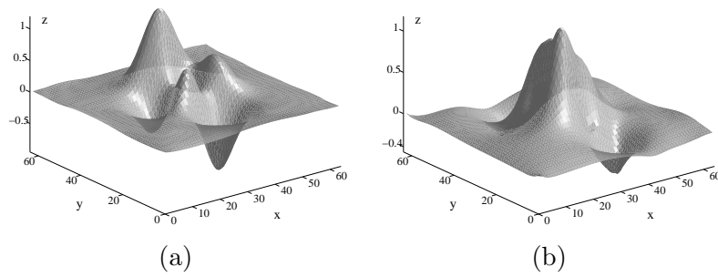
Figure 15: When \lambda_{\text{int}} = 500 and \lambda_{\text{smo}} = 20 : results obtained by M1 starting (a) from 13(a) and (b) from 14(a).
