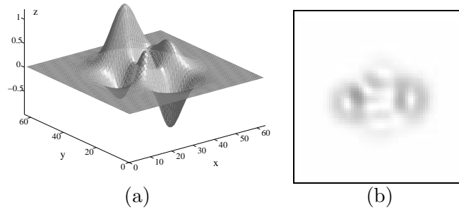
Figure 12: (a) DEM and (b) 64 \times 64 associated image.
