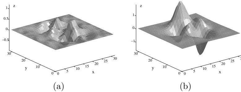
Figure 17: M2 applied to image 12(b): (a) \alpha = 0.99 and (b) \alpha = 0.999998 ( \lambda_{\text{int}} = 500 and \lambda_{\text{smo}} = 20 ).
