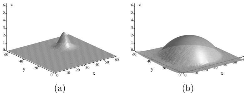
Figure 4: (a) Third starting shape and (b) associated result by M1 ( \lambda_{\text{int}} = 10 and \lambda_{\text{smo}} = 50 ).
