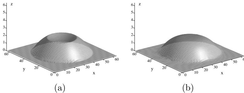
Figure 3: (a) Second starting shape and (b) associated result by M1 ( \lambda_{\text{int}} = 10 and \lambda_{\text{smo}} = 50 ).
