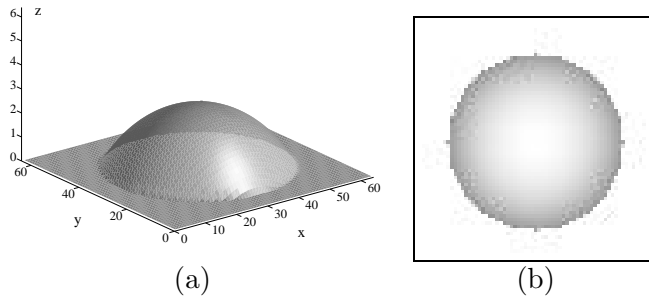
Figure 1: (a) Spherical cap on a background and (b) 64 \times 64 associated image.
