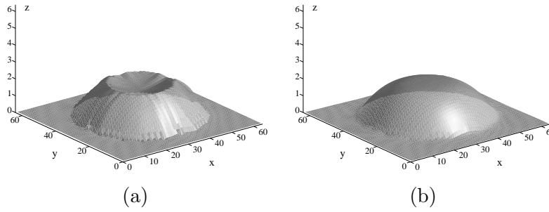
Figure 7: Results obtained by M1 starting from 3(a): (a) \lambda_{\text{int}} = 10 and \lambda_{\text{smo}} = 0 ; (b) \lambda_{\text{int}} = 0 and \lambda_{\text{smo}} = 50 .
