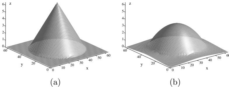
Figure 2: (a) Starting shape and (b) associated result by M1 ( \lambda_{\text{int}} = 10 and \lambda_{\text{smo}} = 50 ).
