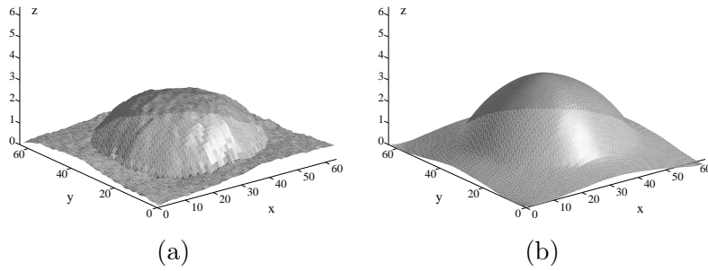
Figure 9: Results obtained by M1 starting from 2(a): (a) \lambda_{\text{int}} = 100 and \lambda_{\text{sno}} = 0 ; (b) \lambda_{\text{int}} = 10 and \lambda_{\text{sno}} = 200 .
