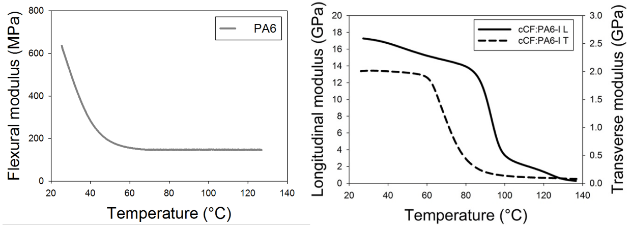
Figure S1 Evolution of (a) the elastic modulus of the PA6, (b) longitudinal and transverse of cCF:PA6-I with temperature.
