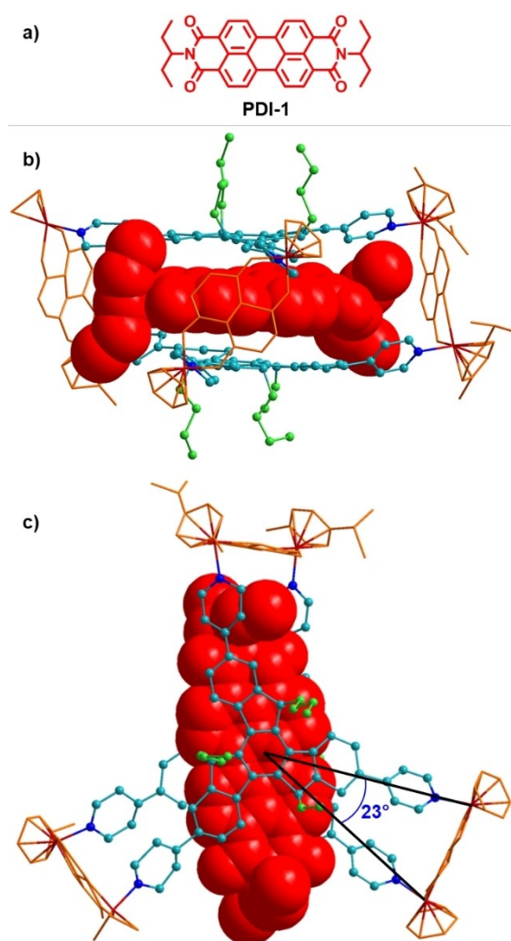
Figure 8. Representation of a) PDI-1 and X-ray crystal structures of PDI-1 \subset\text{Ru}_6\text{Lc}_2 , b) side view, and c) top view (with the corresponding Bailar angle).
