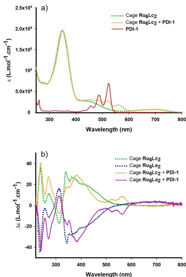
Figure 10. a) UV/Vis absorption spectra of cage \text{Ru}_6\text{Lc}_2 , a stoichiometric mixture of cage \text{Ru}_6\text{Lc}_2 and PDI-1 , PDI-1 , and b) UV/Vis circular dichroism spectra of cages \text{Ru}_6\text{Lc}_2 and \text{Ru}_6\text{La}_2 , and stoichiometric mixtures of cage \text{Ru}_6\text{Lc}_2 and PDI-1 , and cage \text{Ru}_6\text{La}_2 and PDI-1 , in methanol at C=10^{-5} M.
