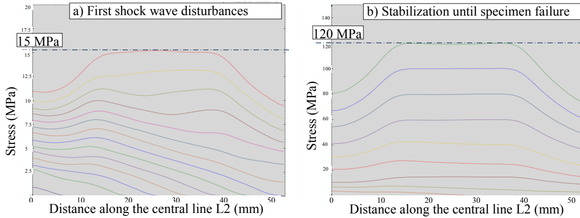
Figure 3. Spatio-temporal profile of the longitudinal stress ( \sigma_{11} ) calculated along the central line of the composite specimen at 0°/90° vs. time.
