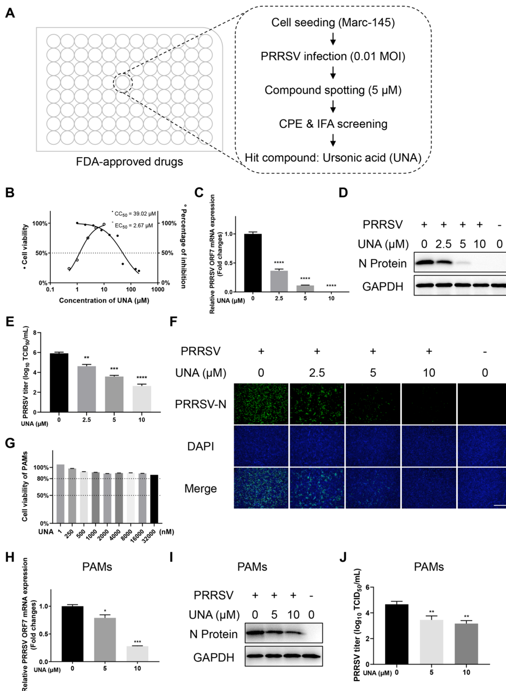
Figure 1 Identification of the anti-PRRSV activity of ursonic acid (UNA) in vitro . A High-throughput screening (HTS) assay flowchart. B 50% cytotoxic concentration ( CC_{50} ) and 50% effective concentration ( EC_{50} ) of UNA in Marc-145 cells. C Relative PRRSV ORF7 mRNA levels in Marc-145 cells determined by RT-qPCR. GAPDH was used as the internal loading control. D Western blotting of the PRRSV N protein in Marc-145 cells infected with PRRSV and treated with the indicated concentrations of UNA. E Virus titration of samples from Marc-145 cells by TCID_{50} calculation. F IFA images of Marc-145 cells (PRRSV-infected and UNA-treated) at 48 hpi. The PRRSV N protein is green, and the nuclei are blue. Scale bars, 500 \mu m. G Viability of PAMs treated with the indicated concentrations of UNA for 24 h. H Relative PRRSV ORF7 mRNA levels in PAMs determined by RT-qPCR. \beta -Actin was used as the internal loading control. I Western blot of the PRRSV N protein in PAMs infected with PRRSV and treated with UNA or DMSO at 24 hpi. J Virus titration of samples from PAMs by TCID_{50} calculation. The results are from one of three independent experiments. The data are presented as the means \pm SDs. The asterisks in the figures indicate significant differences (*, P < 0.05 ; **, P < 0.01 ; ***, P < 0.001 ; ****, P < 0.0001 ; ns, not significant).
