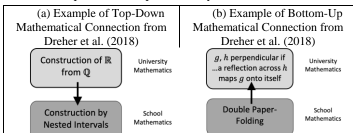
Figure 1. Examples of (a) top-down and (b) bottom-up mathematical connections
