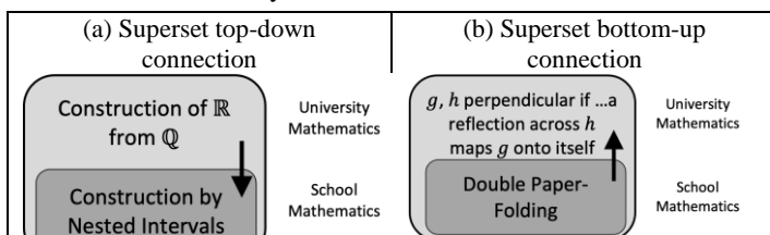
Figure 3. Dreher et al.’s (2018) (a) top-down and (b) bottom-up examples, as superset connections
