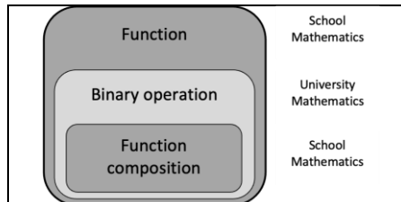
Figure 5. Possible superset and subset mathematical connections for binary operation
