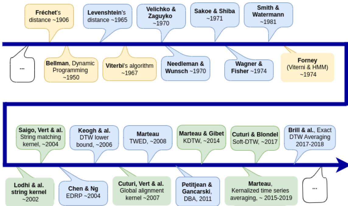
Figure 1: A non exhaustive history of time elastic matching for time series comparison. The founding work is presented in orange, the work on elastic distances in blue and the work on elastic kernel in green.
